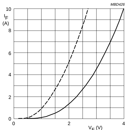
BYM26F and G Dotted line: T_j = 175\text{ °C} . Solid line: T_j = 25\text{ °C} .
