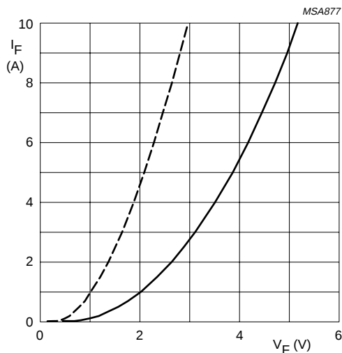
BYM26A to E Dotted line: T_j = 175\text{ °C} . Solid line: T_j = 25\text{ °C} .
