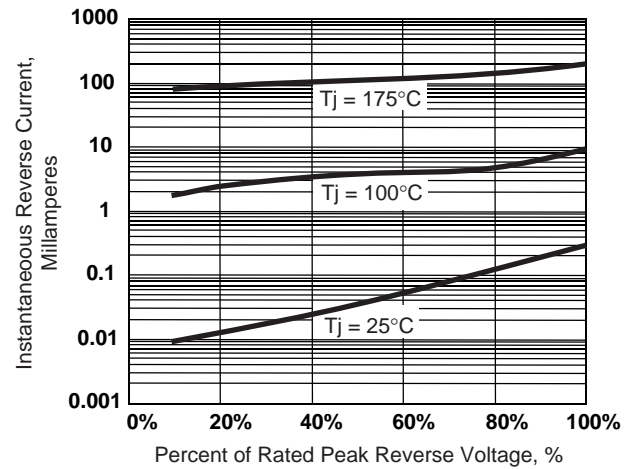
Figure 4 – MUR460 Typical Reverse Characteristics
