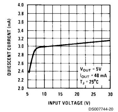
Quiescent Current
