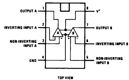
Dual-In-Line Package
