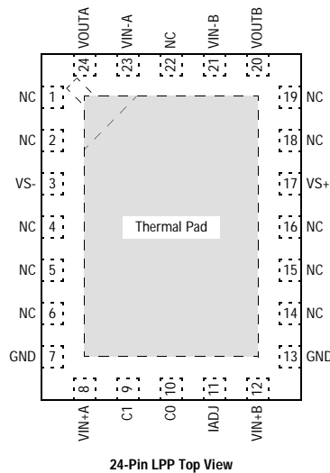
Pin Configurations continues on Page 3
