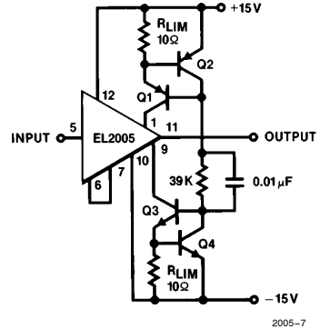
Current Limiting Using Current Sources
