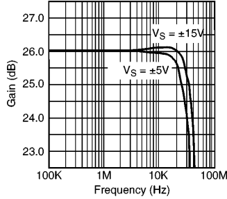
Gain Flatness V_S = \pm 5V , A_V = 26 dB, R_F = 680\Omega , R_G = 36\Omega
