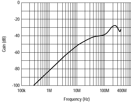
Channel-to-Channel Isolation vs Frequency
