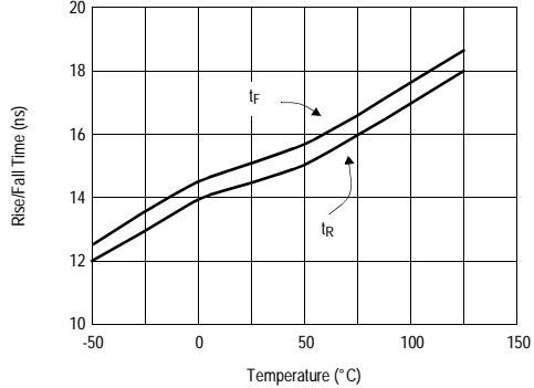
Rise/Fall Time vs Temperature C_{\text{L}} = 2000\text{pF}, V_{\text{S+}} = 15\text{V}
