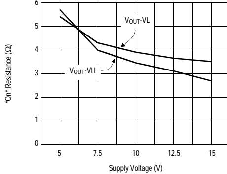
"On" Resistance vs Supply Voltage I_{\text{OUT}} = 200\text{mA}, T = 25^\circ\text{C}, V_{S+} = V_{\text{H}}, V_{\text{L}} = 0\text{V}
