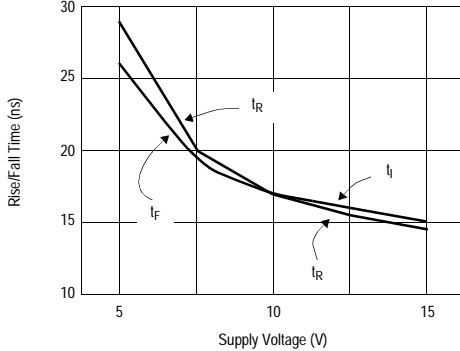
Rise/Fall Time vs Supply Voltage C_{\text{L}} = 2000\text{pF}, T = 25^\circ\text{C}
