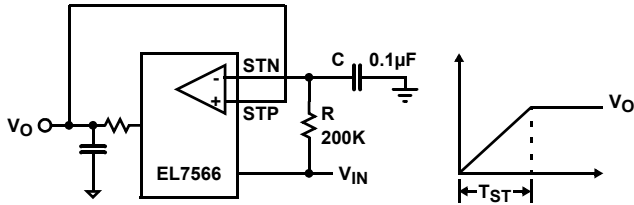
FIGURE 21. ADJUSTABLE START-UP
