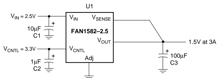
Figure 5. Application Circuit (FAN1582-2.5)
