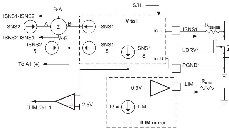
Figure 6. Current Limit and Active Droop Circuits
