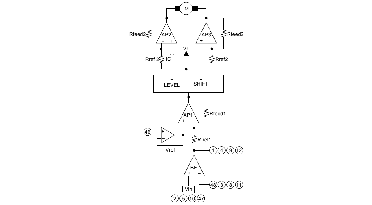
Figure 1. Regulator circuit
