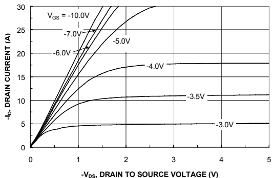
Figure 11. On-Region Characteristics.
