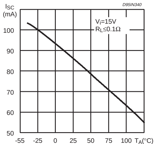
Figure 8: Reference Short Circuit Current vs. Temperature.
