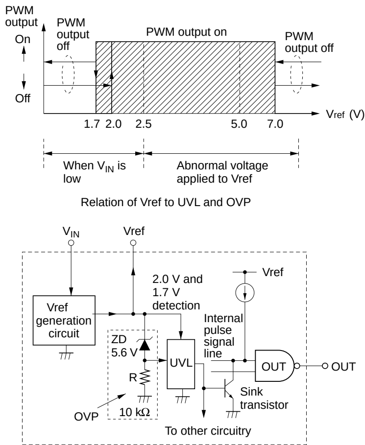
Figure 5.1 Quick Shutoff
