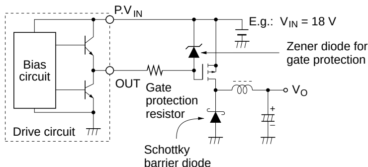
Figure 4.1 P-channel Power MOS FET (example)
