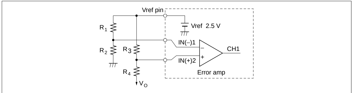
Figure 2.1 Inverting Output
