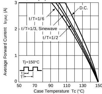
T C – I F(AV) Characteristics
