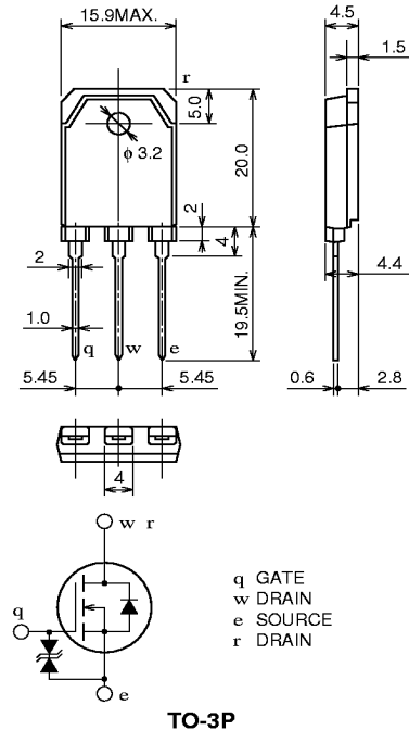
OUTLINE DRAWING
