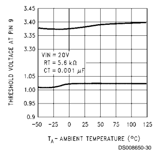
Maximum & Minimum Duty Cycle Threshold Voltage
