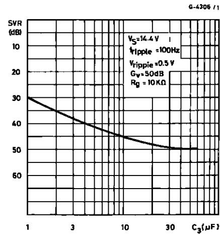
Figure 15 : Supply Voltage Rejection versus C3 (Stereo amplifier)
