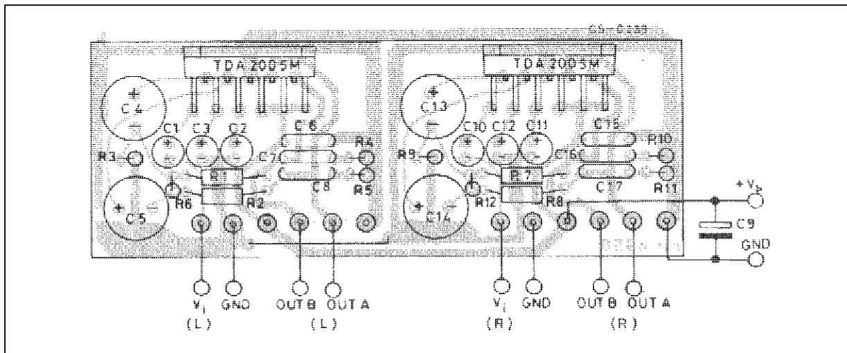
Figure 26 : P.C. Board and Components Layout of Figure 25 (1:1 scale)
