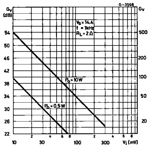
Figure 20 : Gain versus Input Sensitivity (Stereo amplifier)
