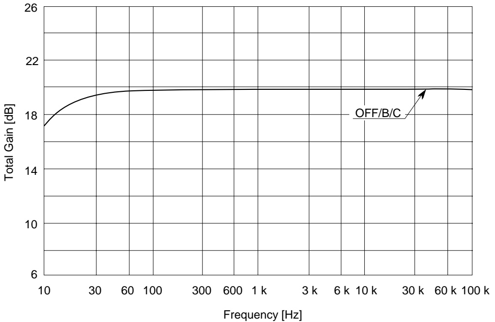
Total Gain vs. Frequency (PB MODE RECOUT V_{cc} = 14\text{ V} )
