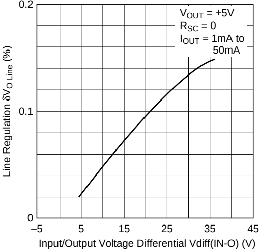
Line Regulation vs. Input/Output Voltage Differential-2
