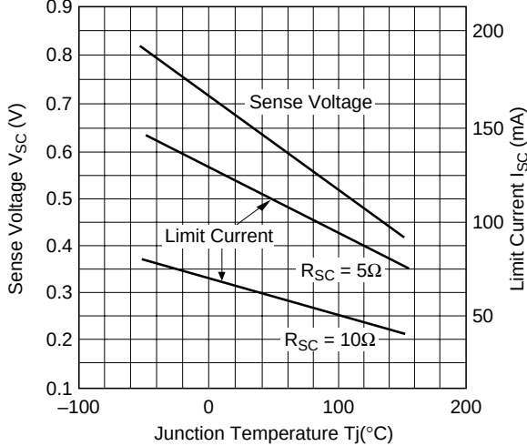
Current Limiting Characteristics
