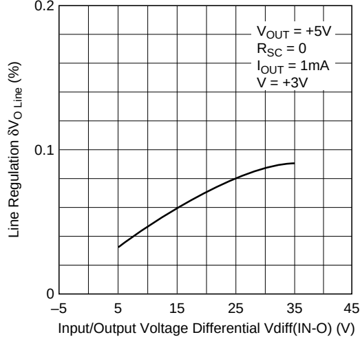
Line Regulation vs. Input/Output Voltage Differential-1
