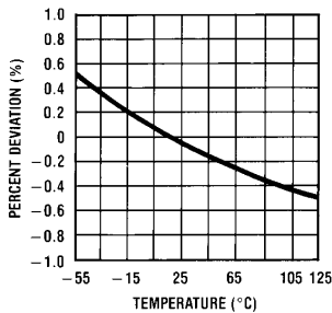
Typical 1ms Pulse Width Variation vs. Temperature
