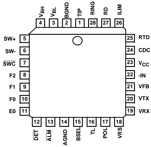
HC55185 (PLCC) TOP VIEW
