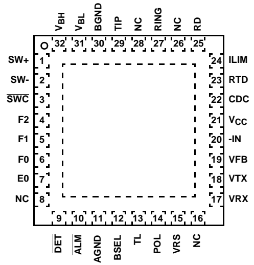
HC55185 (QFN) TOP VIEW
