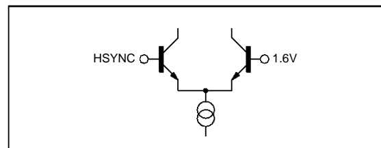
Figure 7 : Input Structure
