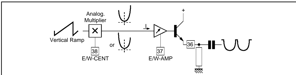
Figure 22 : Vertical Part Block Diagram
