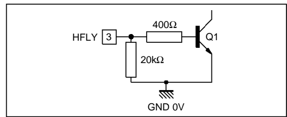
Figure 16 : Flyback Input Electrical Diagram
