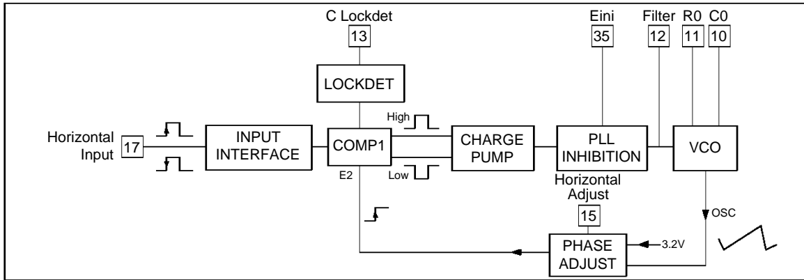
Figure 8 : Principle Diagram
