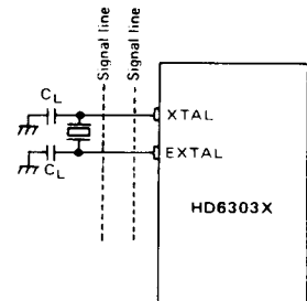
Figure 26 Warning concerning board design of oscillation circuit
