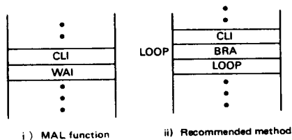
Figure 29 Program to wait for interrupt
