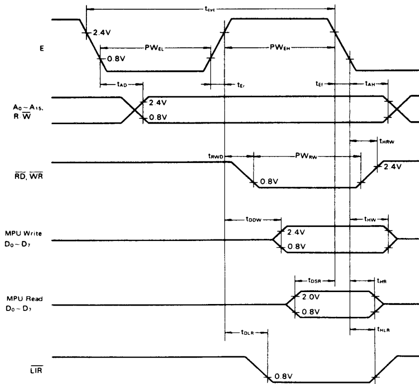
Figure 1 Bus Timing
