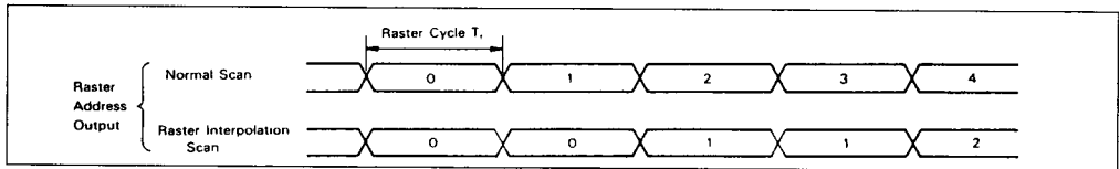
Figure 15 Raster Address Output and Raster Interpolation
