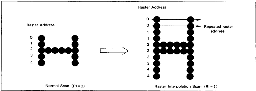
Figure 14 Raster Interpolation
