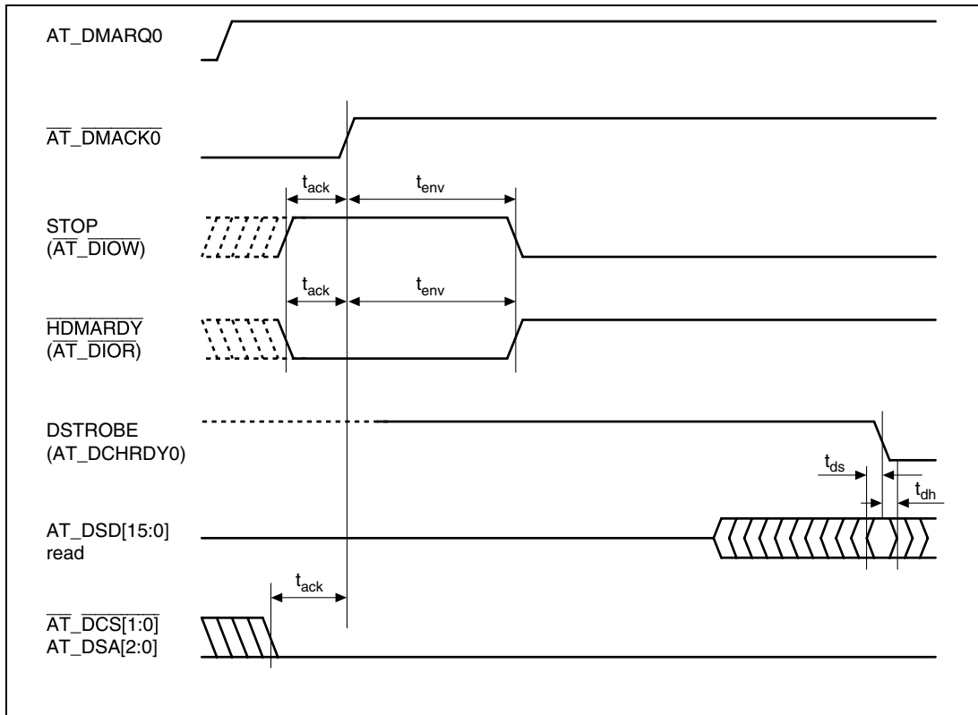
Figure 31.25 Initiating an Ultra DMA Data-in Burst
