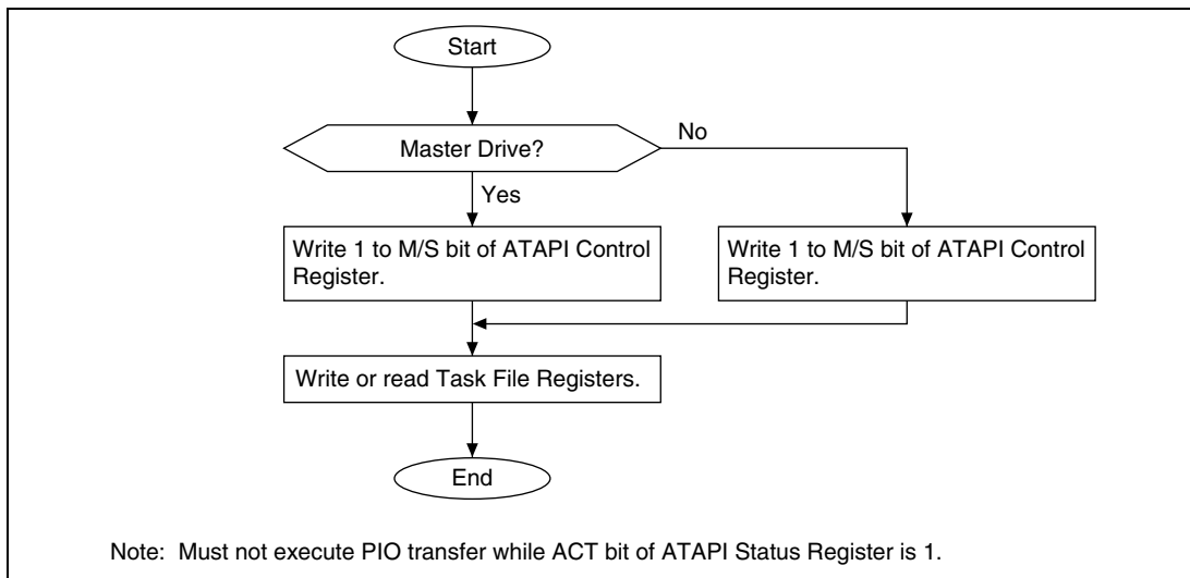
Figure 18.6 Procedure in PIO Transfer Mode (Not Using FIFO)
