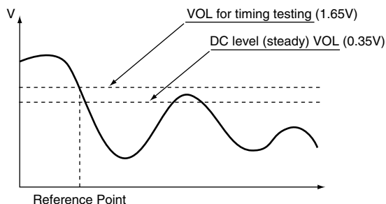
Figure 31.53 Timing Testing
