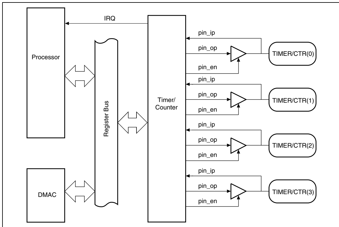
Figure 26.1 Timer Interface Block Diagram.
