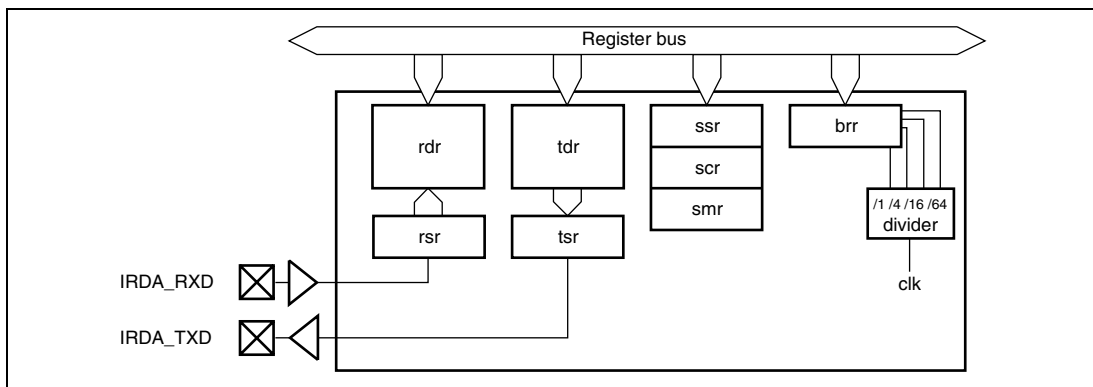
Figure 22.2 Functional Block Diagram
