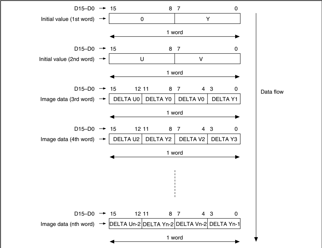
Figure 12.3 DELTA YUV Data Format
