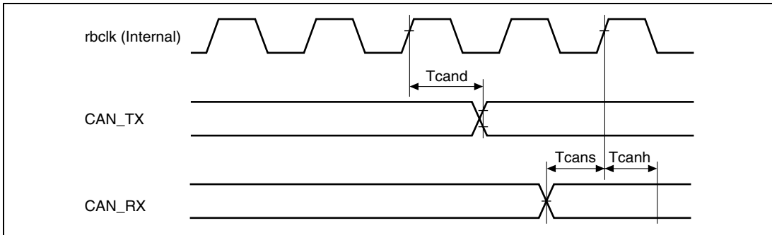
Figure 31.20 CAN Timing
