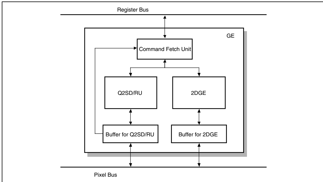
Figure 11.1 GE Block Diagram
