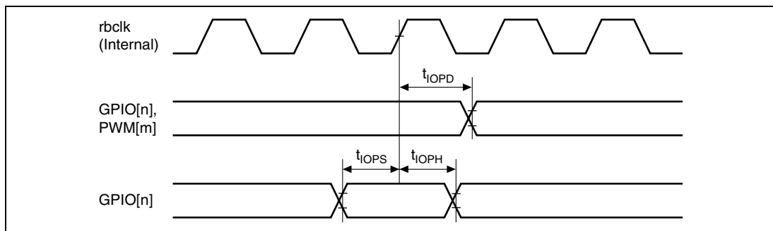
Figure 31.16 GPIO, PWM Timing
