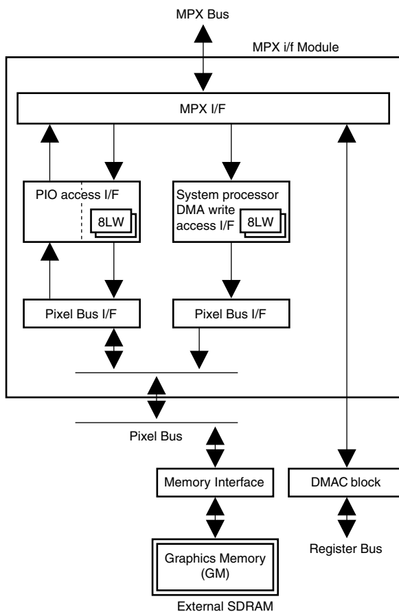
Figure 3.1 Block Diagram
