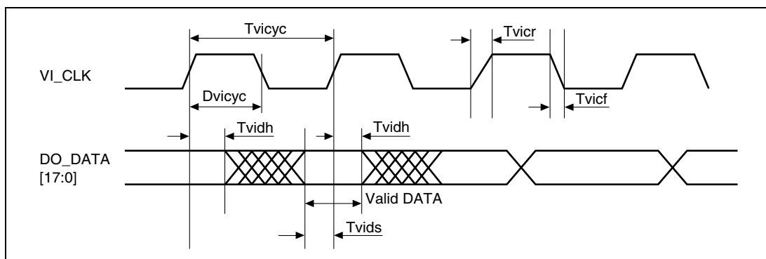
Figure 31.15 Video In Timing
