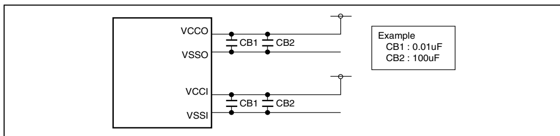
Figure 31.55 Notes on Power Supply
