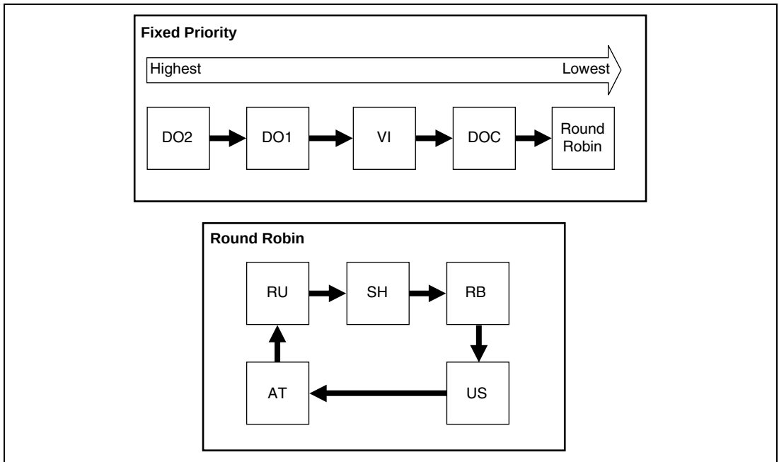
Figure 7.1 Arbitration Diagram
