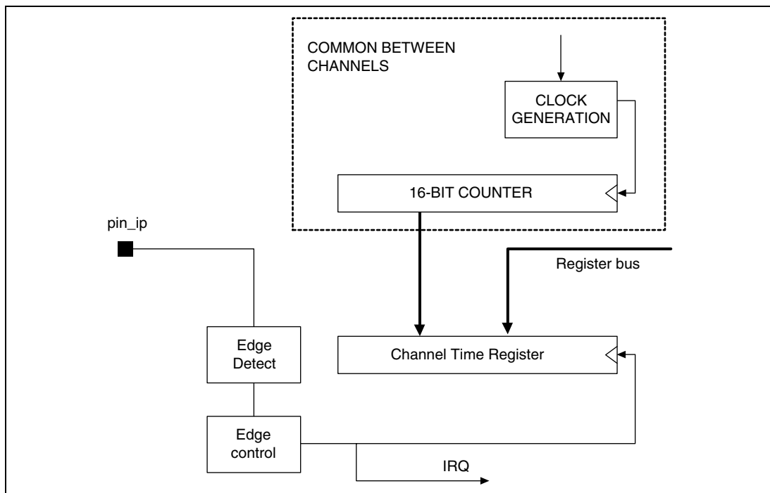
Figure 26.6 16 bit Timer Mode: Input captureS
