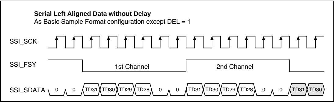
Figure 14.15 Serial Left Aligned without Delay
