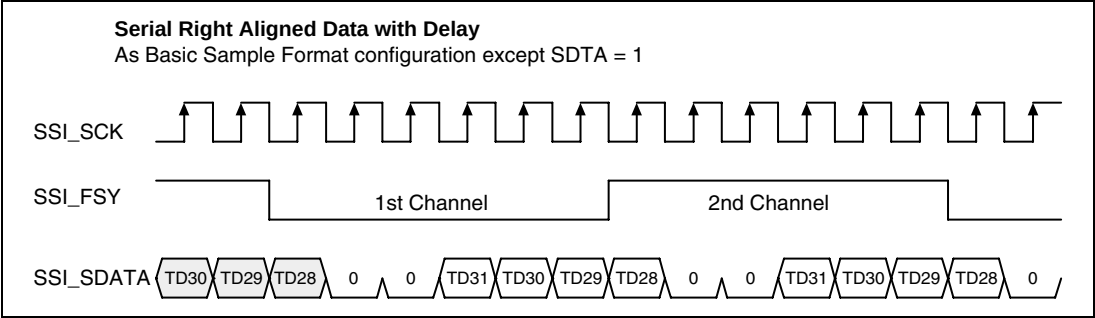
Figure 14.13 Serial Right Aligned with Delay
