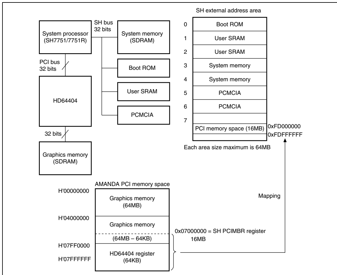
Figure 1.8 PCI System Example
