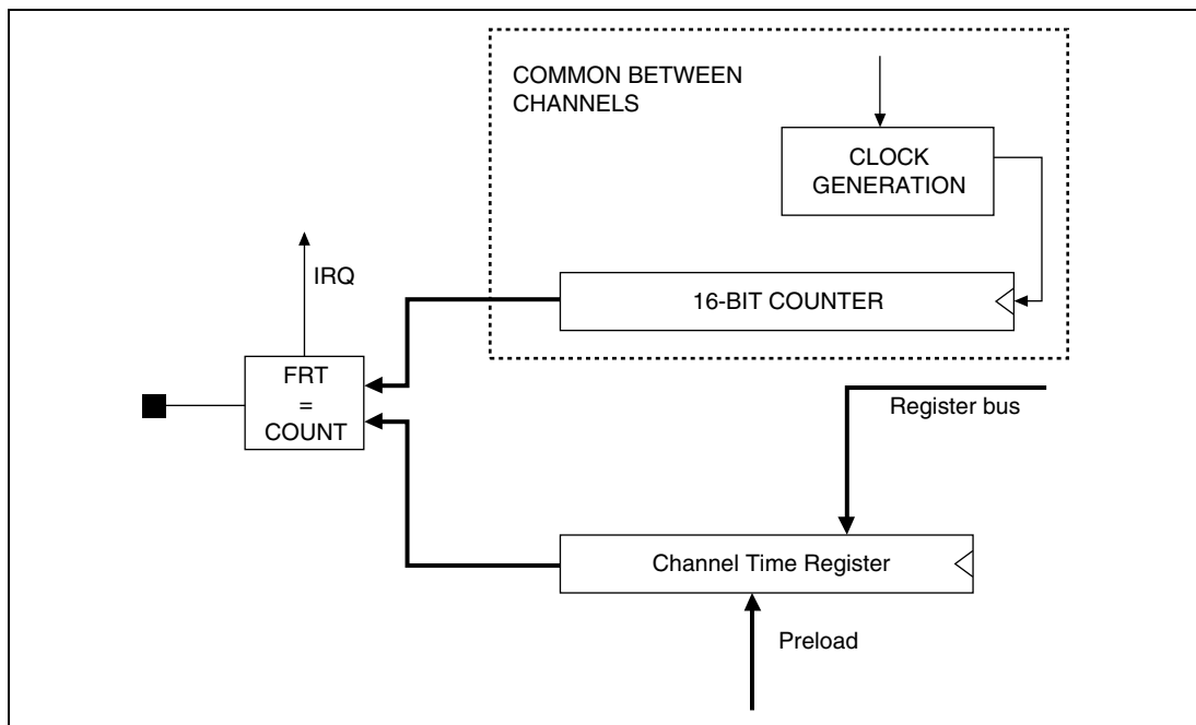
Figure 26.7 16 bit Timer Mode: Output Compare
