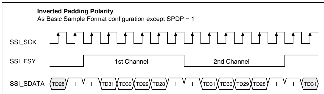
Figure 14.12 Inverted Padding Polarity
