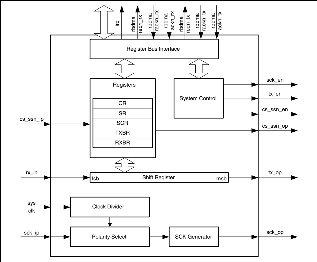
Figure 17.5 Functional Diagram
