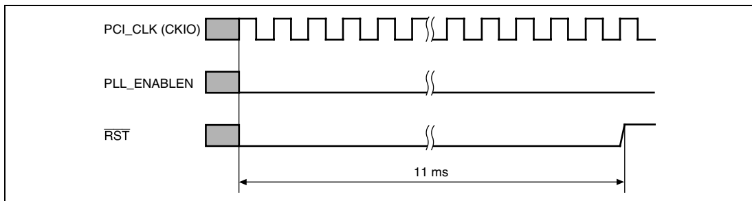
Figure 8.2 Power-On Sequence Timing
