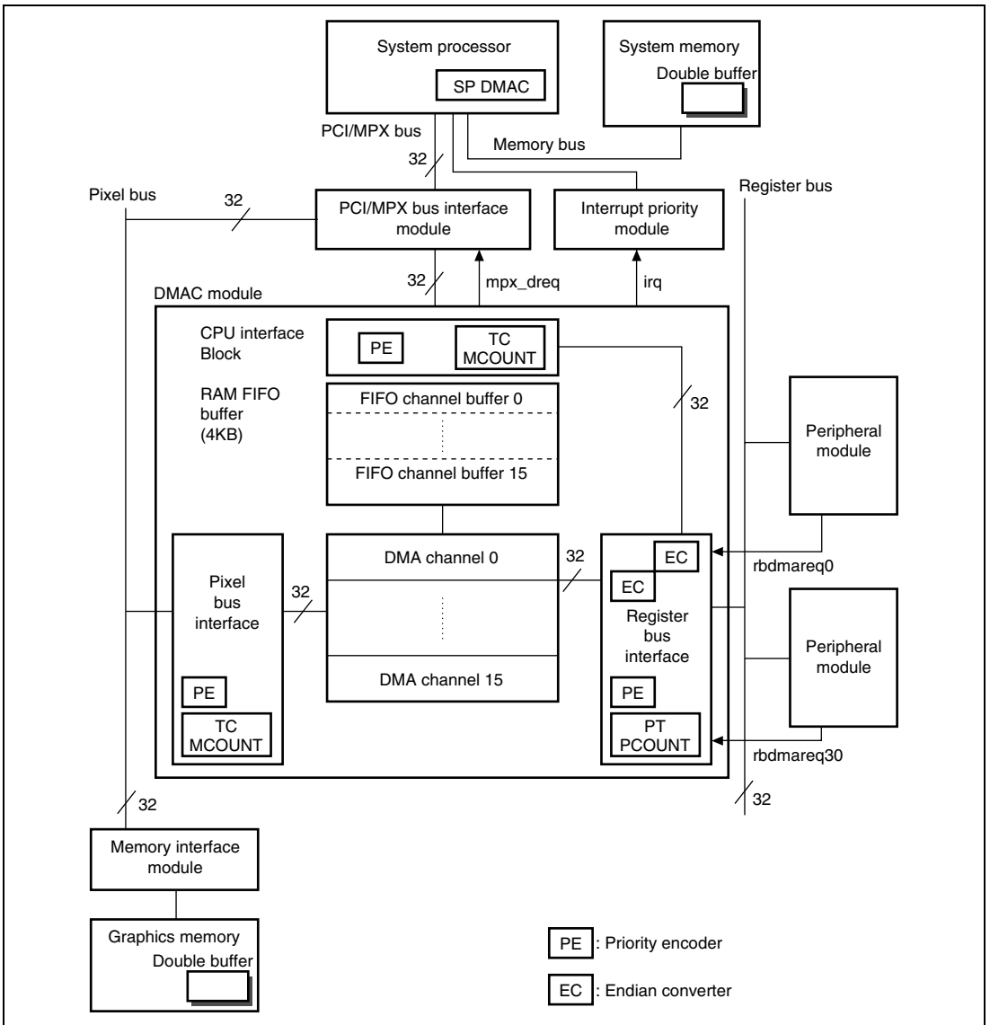
Figure 2.1 System Diagram
