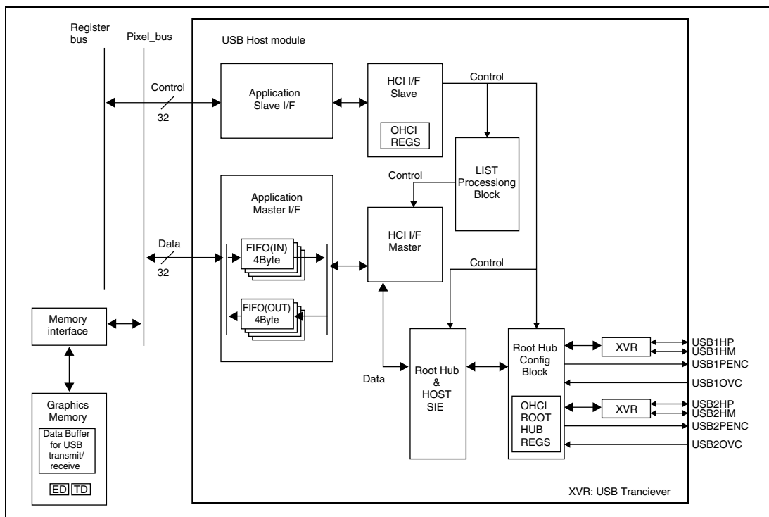
Figure 24.1 Block Diagram of USB Host
