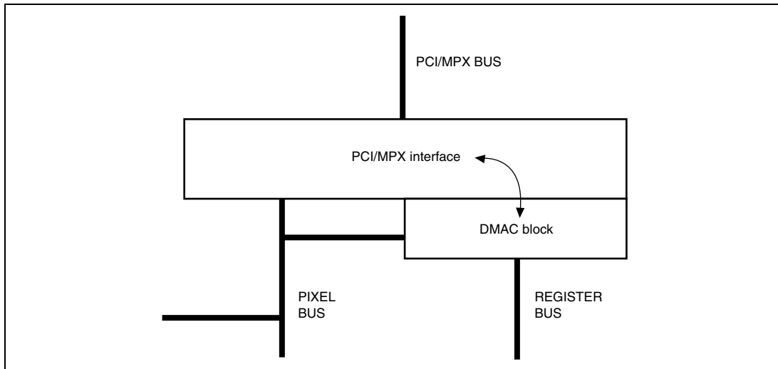
Figure 1.5 System Interface
