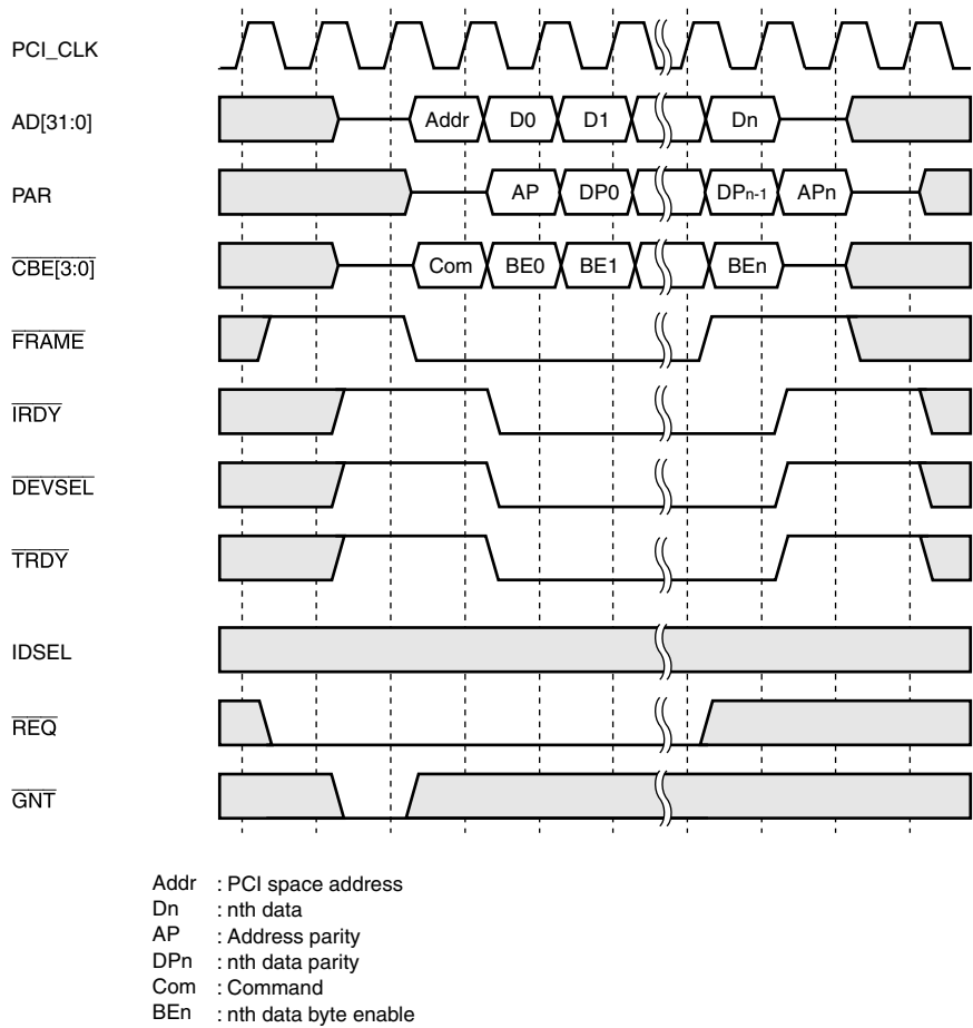
Figure 4.3 Master Memory Write Cycle in Non-Host Mode (Burst)
