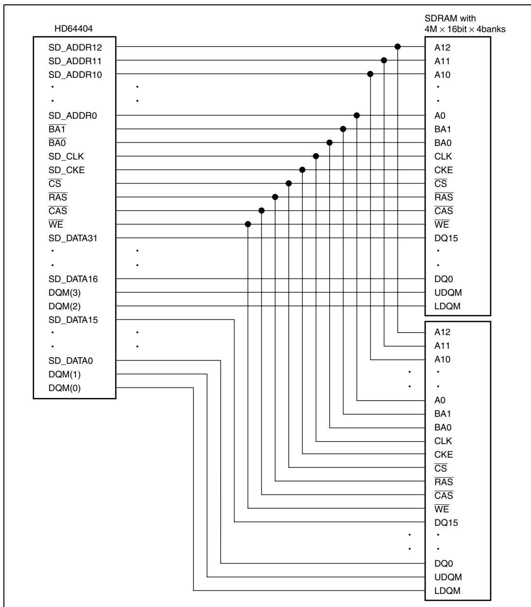
Figure 6.1 Example of Connection of 256-Mbit 16-bit Synchronous DRAM
