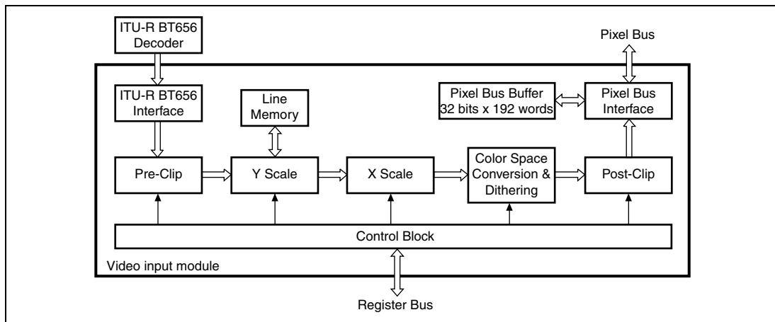
Figure 9.1 System Diagram
