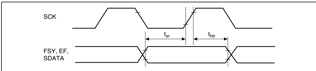
Figure 31.37 Timing for SSI Receiver (1)
