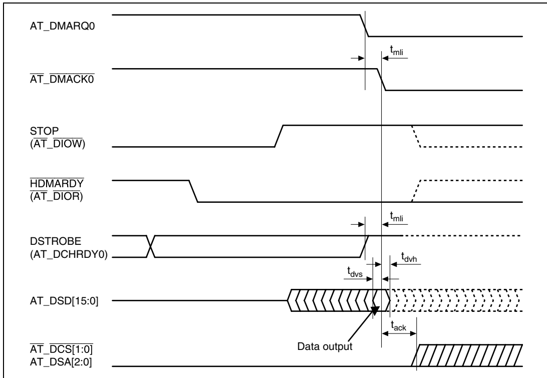
Figure 31.28 Host Terminating an Ultra DMA Data-in Burst
