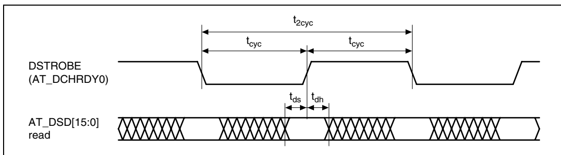
Figure 31.26 Sustained Ultra DMA Data-in Burst
