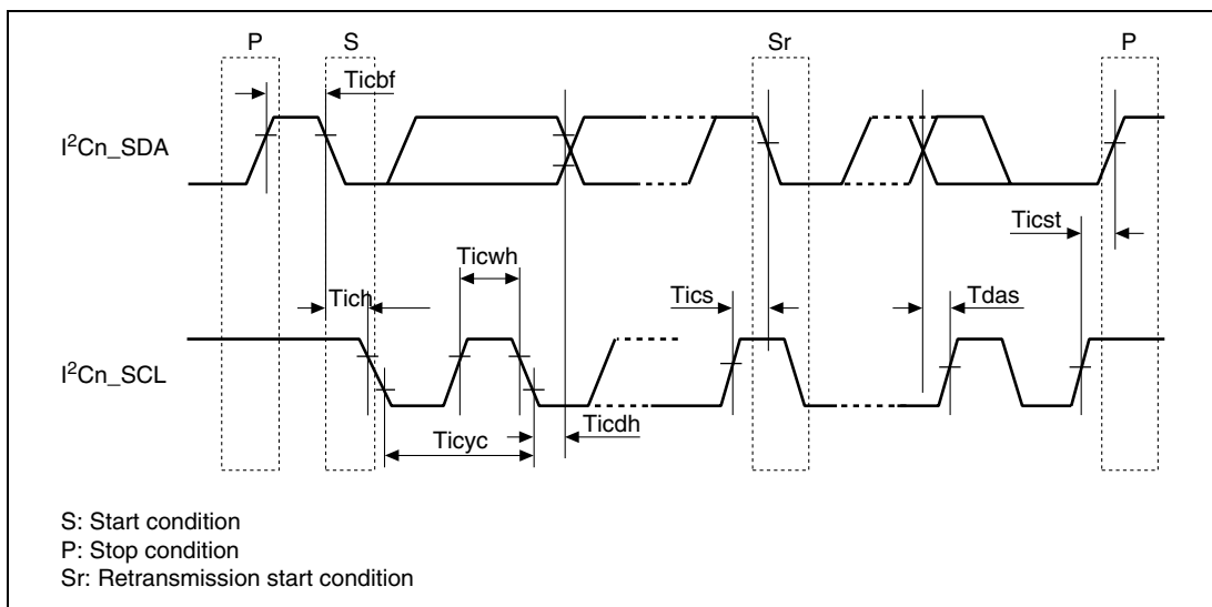
Figure 31.22 I 2 C Timing
