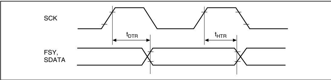
Figure 31.35 Timing for SSI Transmitter (1)
