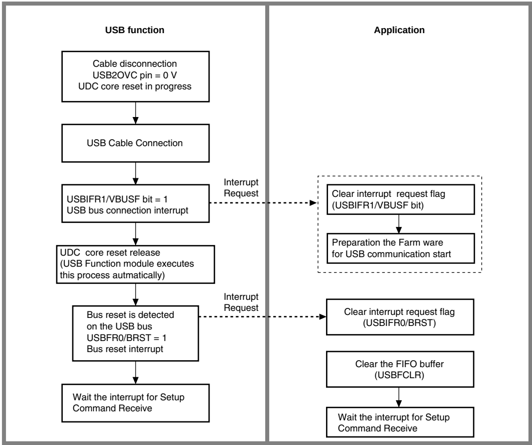
Figure 23.2 Cable Connection Operation
