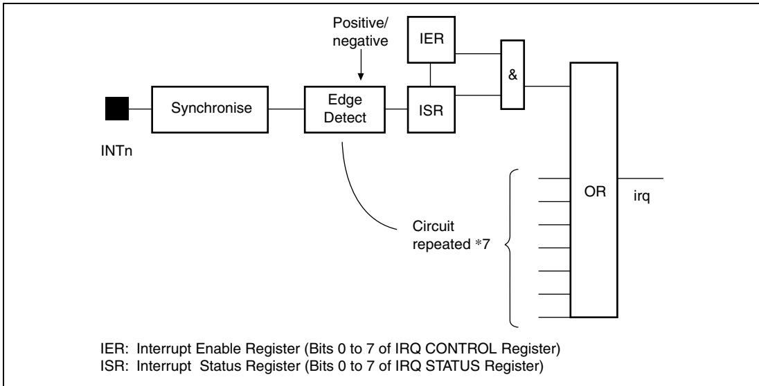
Figure 25.1 Interrupt Input Block Diagram
