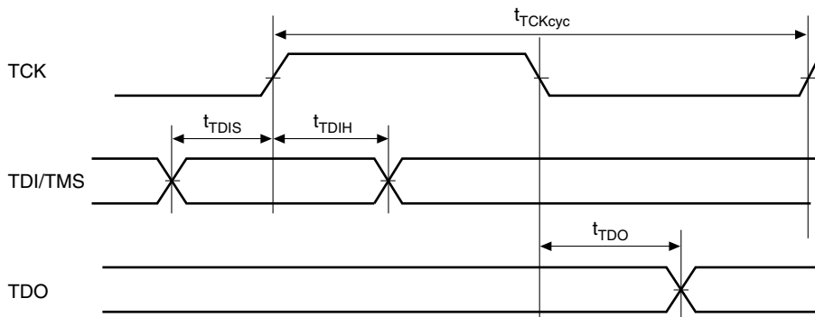
Figure 31.52 JTAG Data Transfer Timing
