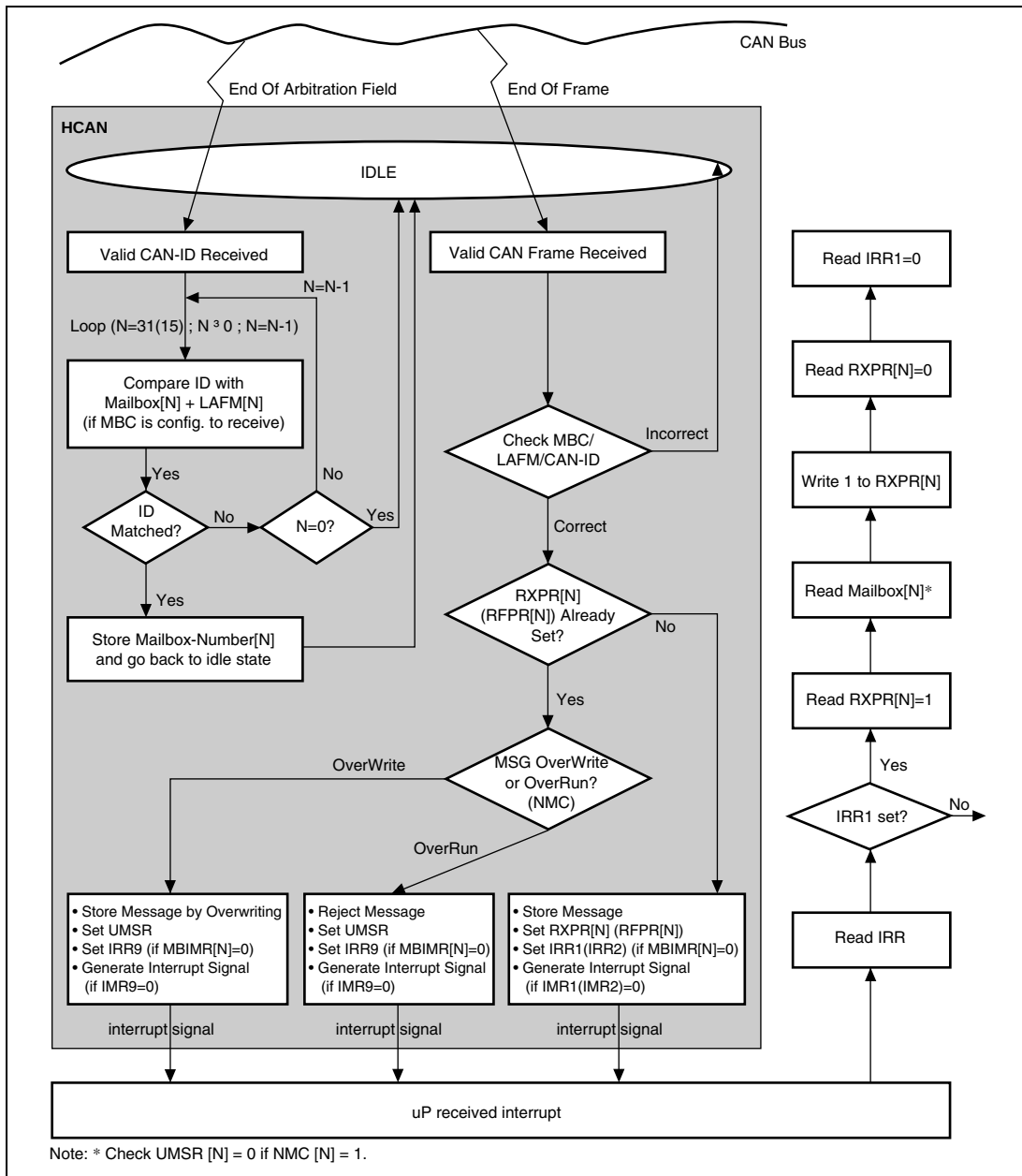
Figure 19.12 Message Receive Sequence
