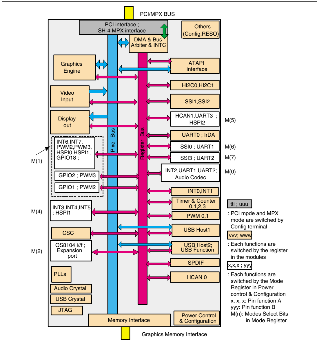
Figure 1.1 HD64404 Block Diagram
