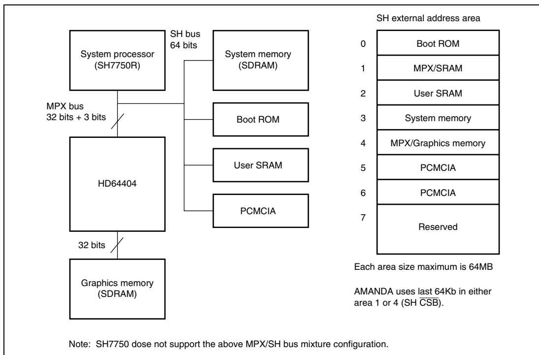
Figure 1.6 MPX System Example 1
