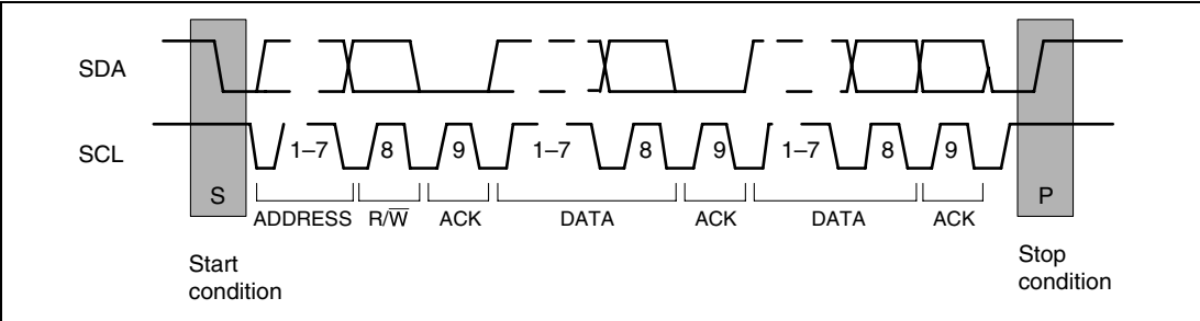
Figure 16.3 I 2 C Bus Timing
