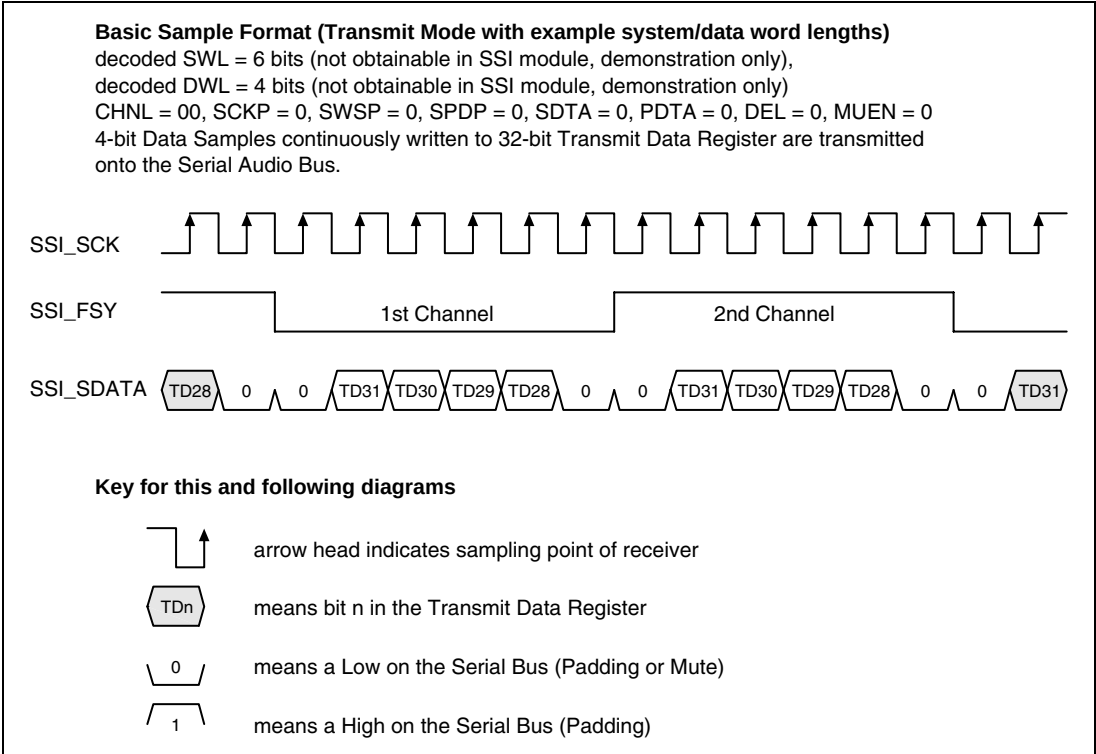
Figure 14.9 Basic Sample Format (Transmit Mode with Example System/Data Word Length)
