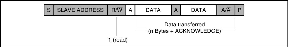
Figure 16.5 Master Data Receive Format
