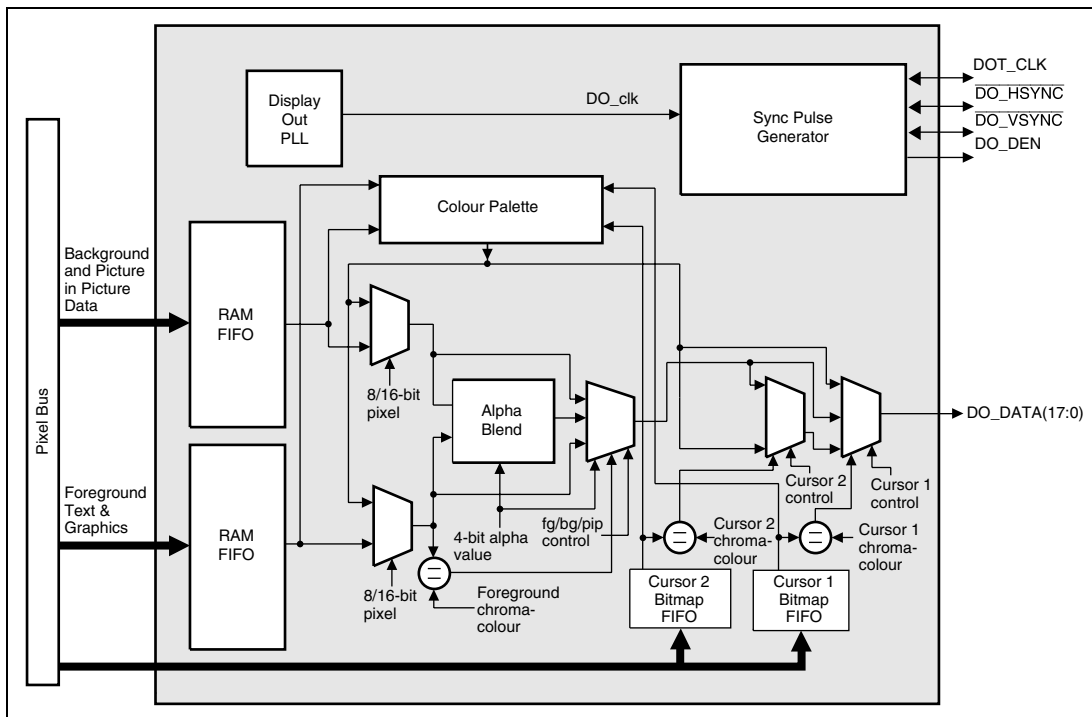
Figure 10.1 Block Diagram
