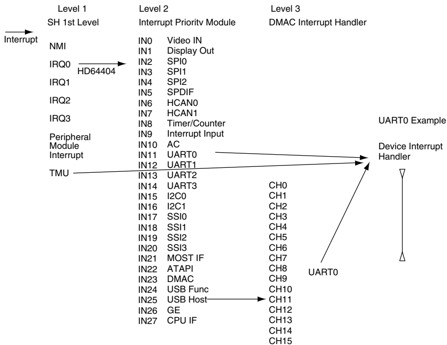
Figure 2.4 Interrupt Handling Hierarchy in HD64404: UART0 Example
