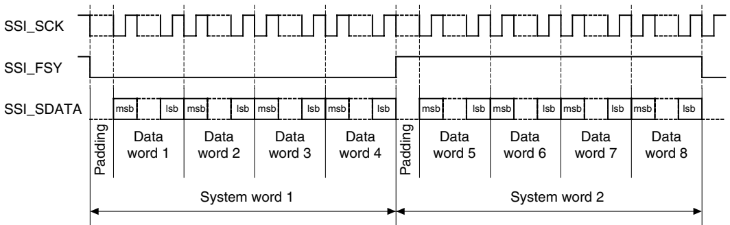
Figure 14.8 Multichannel Format (8 Channels, Right Aligned with Padding)
