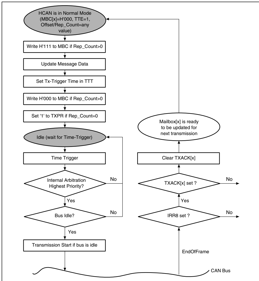
Figure 19.10 Time Triggered Transmission
