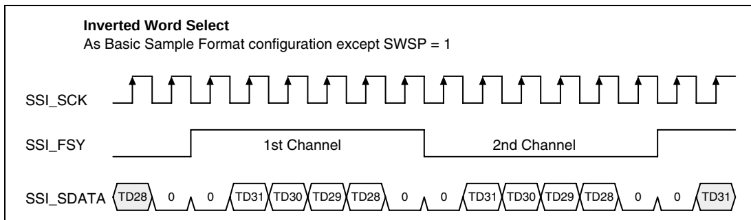
Figure 14.11 Inverted Word Select
