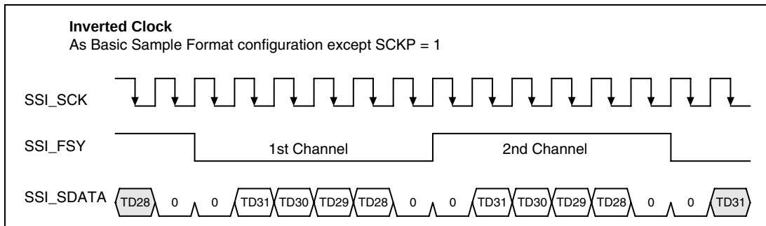
Figure 14.10 Inverted Clock
