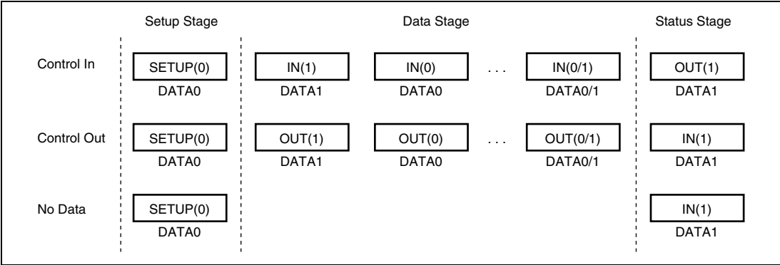
Figure 23.4 Each Transfer Stage in Control Stage
