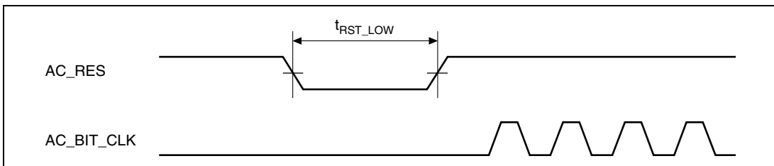
Figure 31.48 Cold Reset Timing
