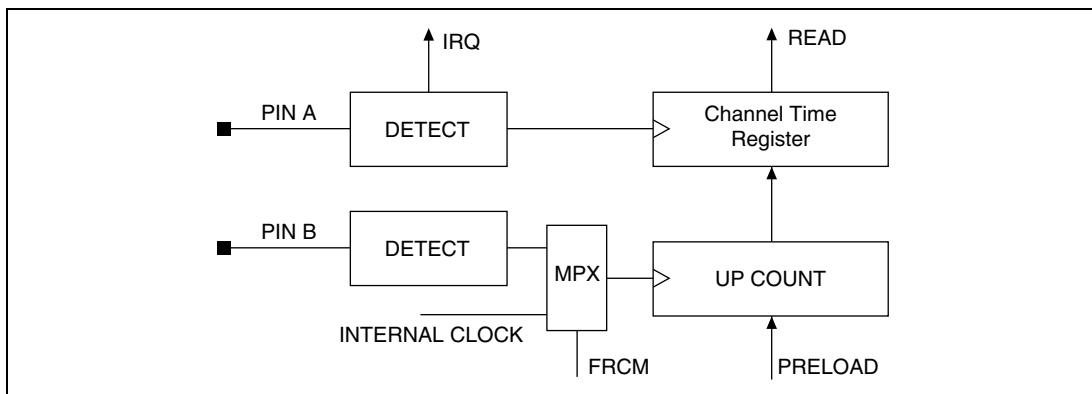
Figure 26.10 Upcounter with Capture Mode
