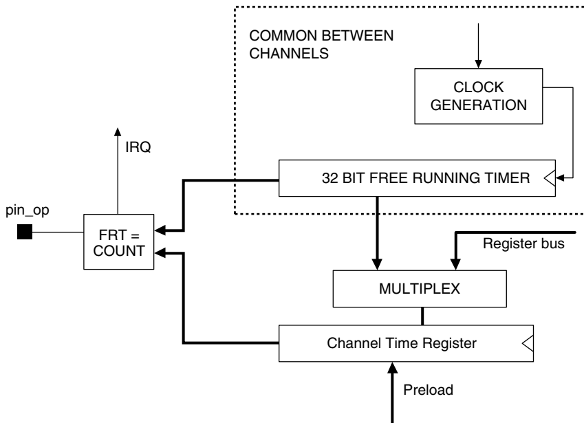
Figure 26.5 32-bit Timer Mode: Output Compare
