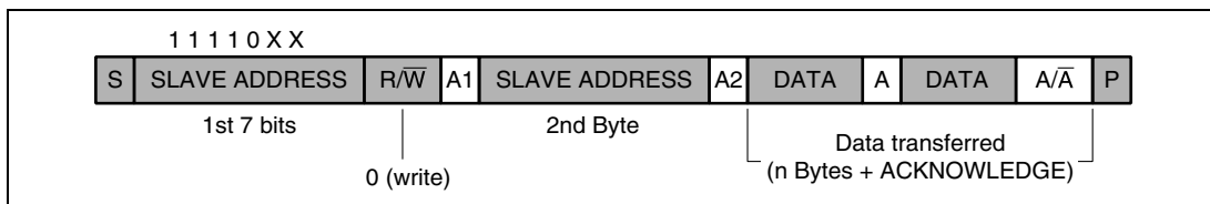
Figure 16.7 10-Bit Address Data Transfer Format
