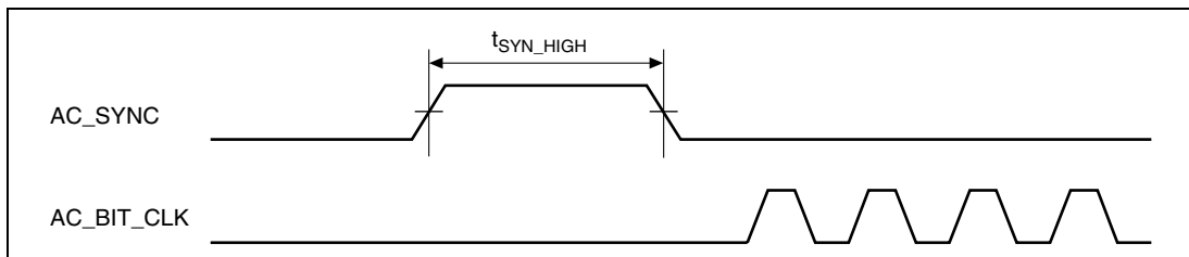
Figure 31.49 Warm Reset Timing
