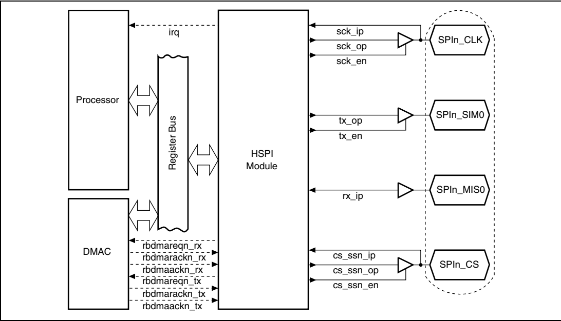
Figure 17.1 Interface Block Diagram
