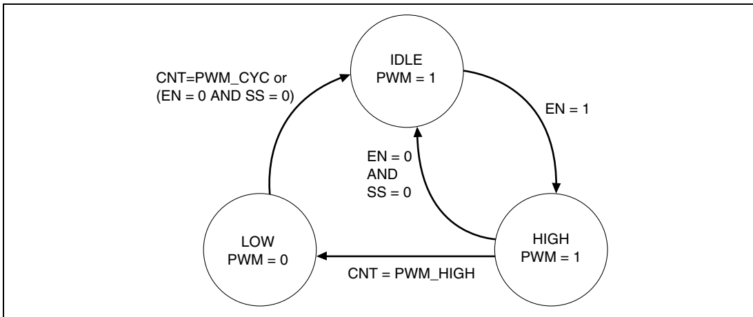
Figure 27.1 PWM State Transition
