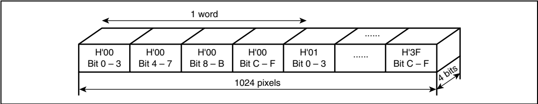
Figure 11.15 Configuration of One Memory Unit (512 Bytes) (2)
