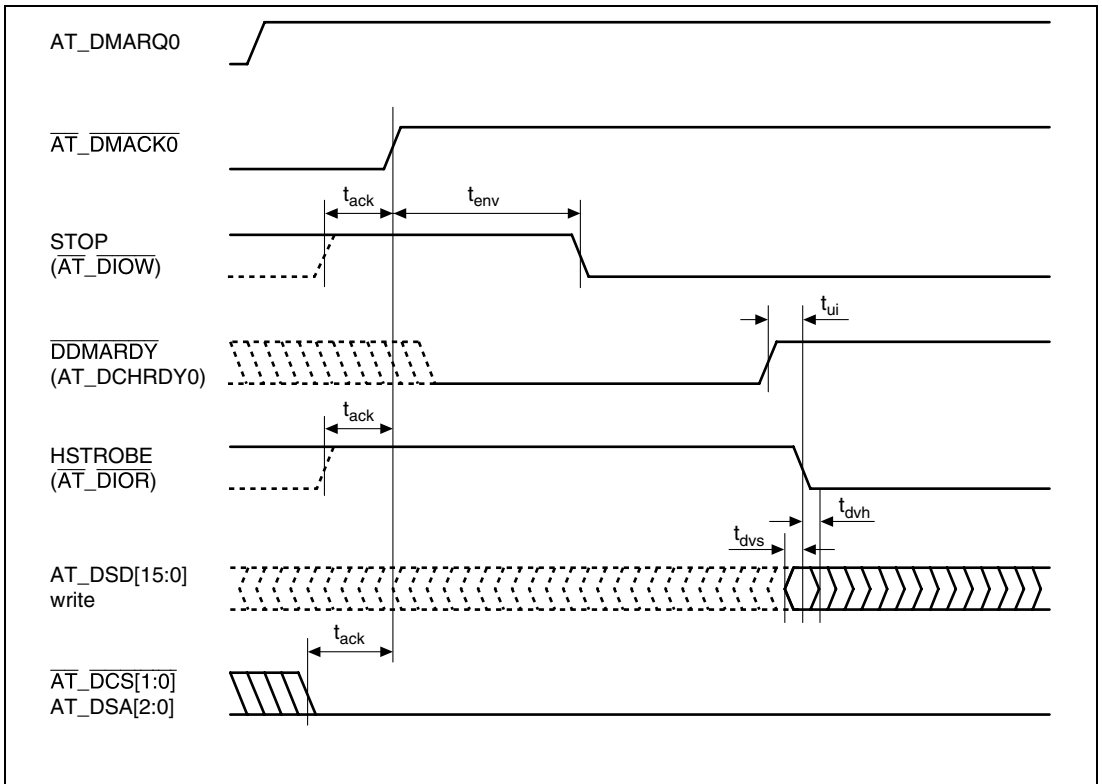
Figure 31.29 Initiating an Ultra DMA Data-out Burst
