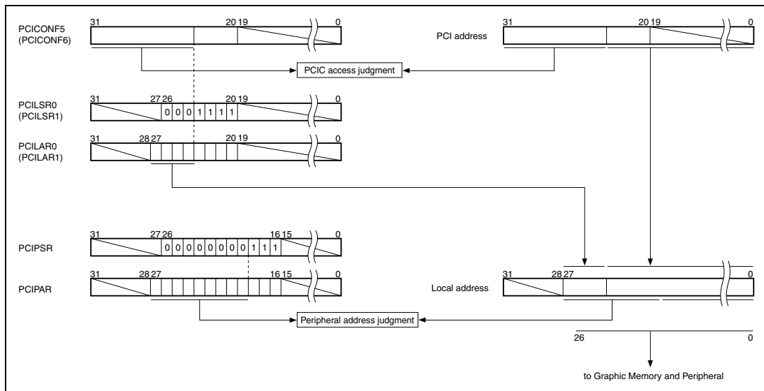
Figure 4.2 Local Address Space
