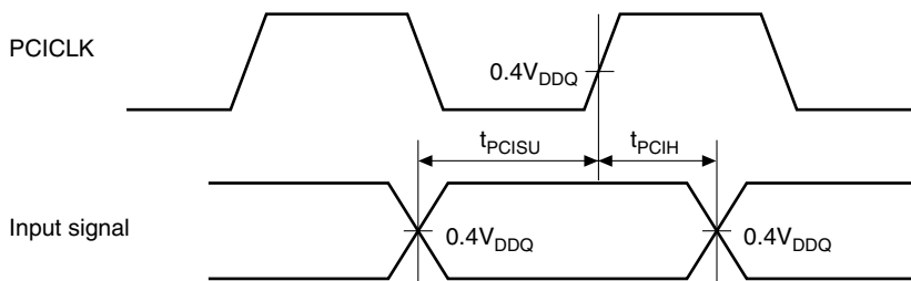
Figure 31.8 Input Signal Timing
