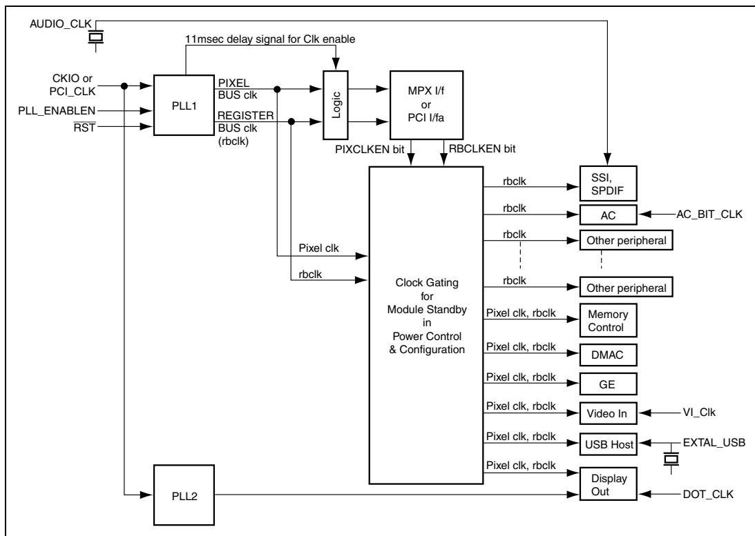
Figure 8.3 Block Diagram of Clock Pulse Generator
