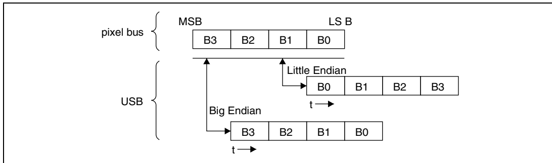
Figure 24.2 Endian Data Flow
