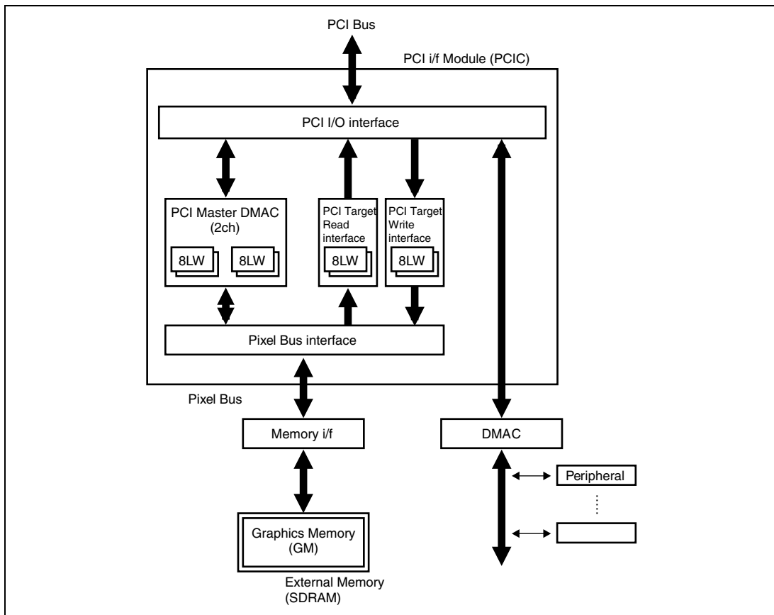
Figure 4.1 Block Diagram
