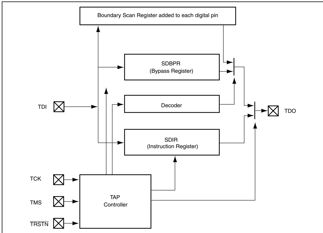
Figure 30.1 Block diagram of HD64404 JTAG Circuit
