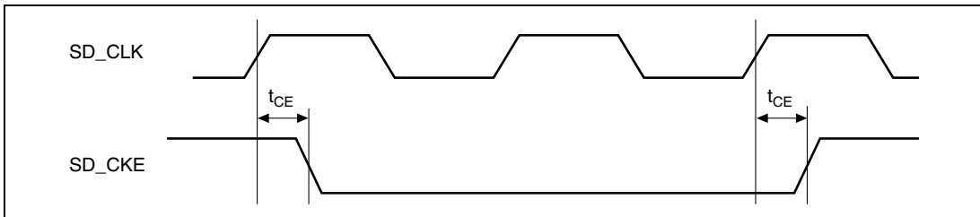
Figure 31.11 SDRAM Clock
