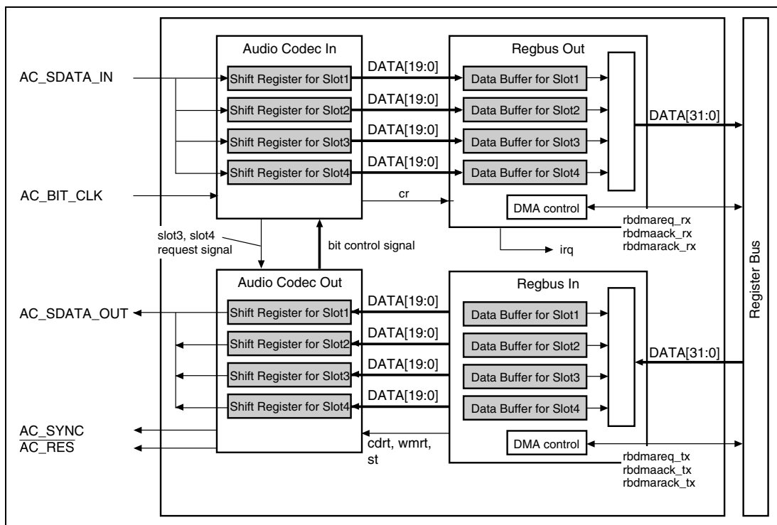
Figure 13.1 Block Diagram
