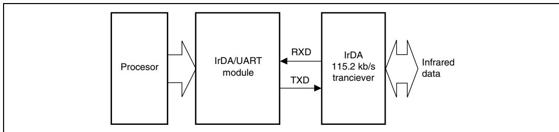
Figure 22.1 Overview Block Diagram
