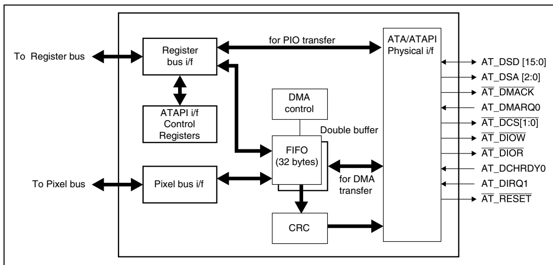
Figure 18.1 ATAPI Block Diagram
