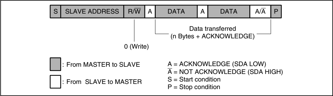
Figure 16.4 Master Data Transmit Format
