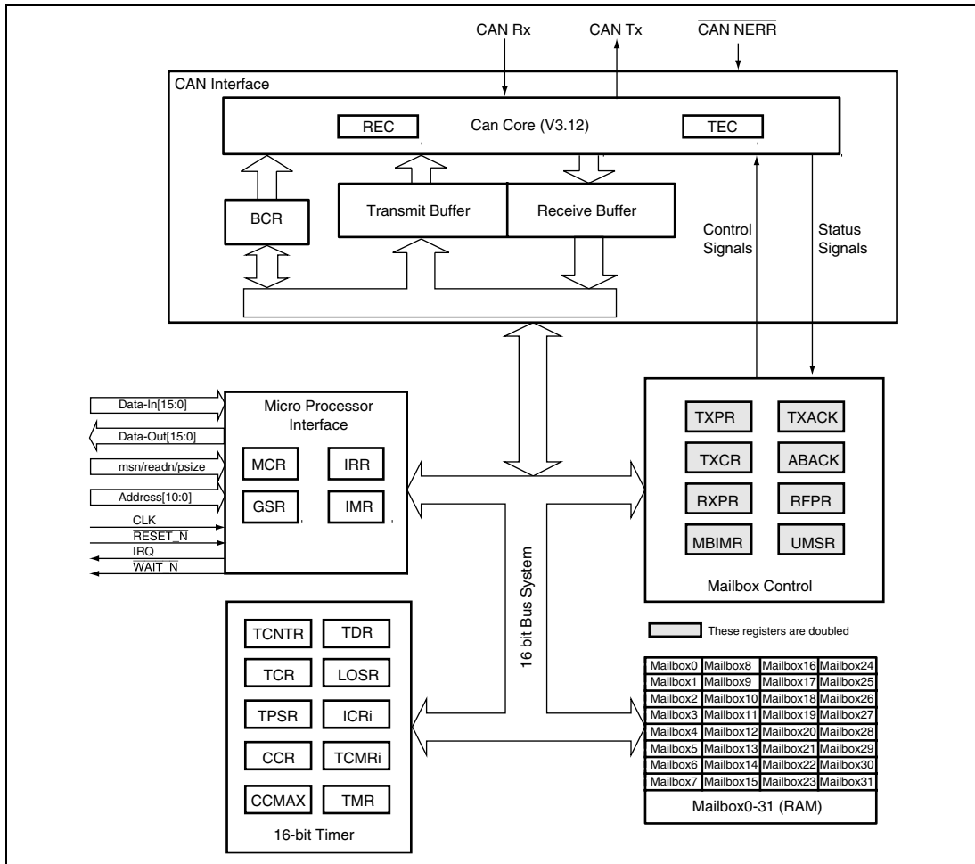
Figure 19.1 Block Diagram of HCAN-2 Module
