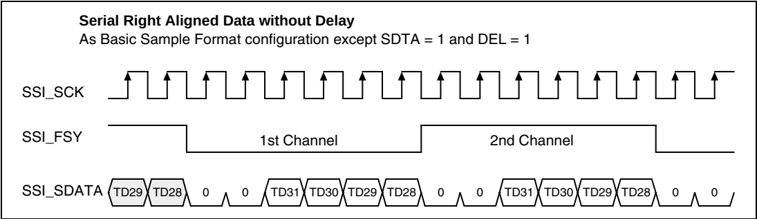
Figure 14.14 Serial Right Aligned without Delay
