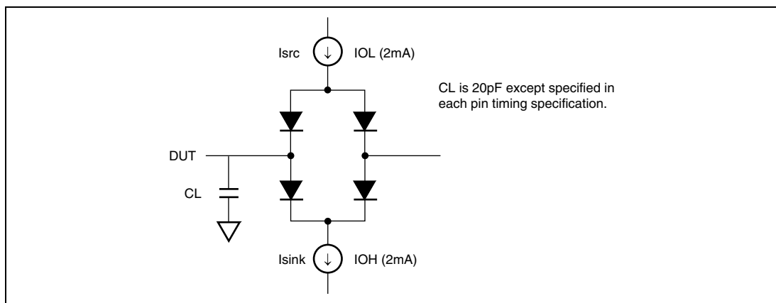
Figure 31.54 Test Load Circuit
