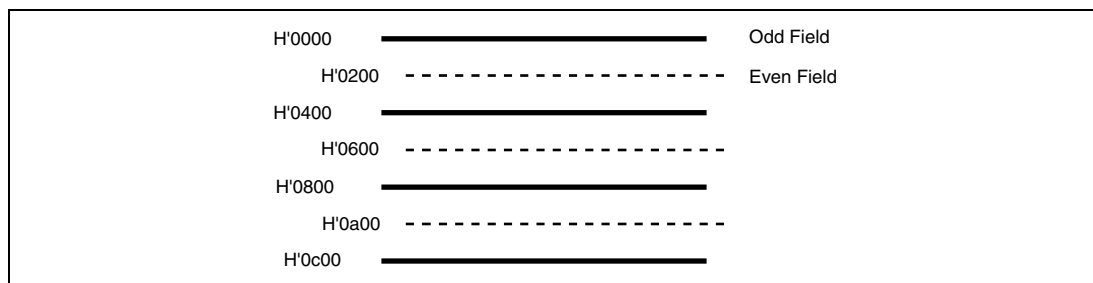
Figure 9.2 Interlaced Frame Memory Interleaving
