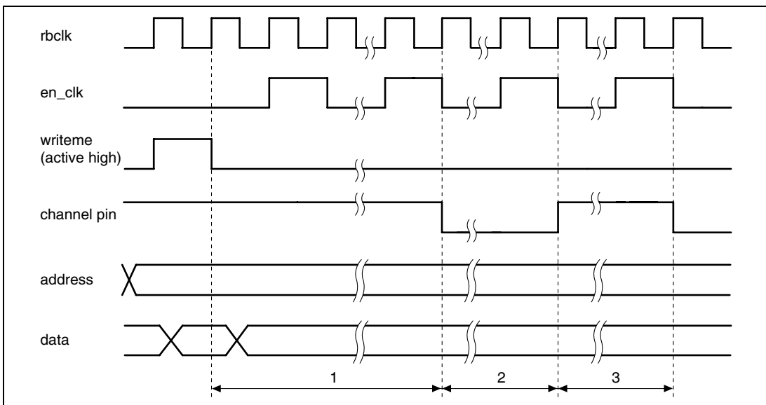
Figure 27.2 PWM Output Timing
