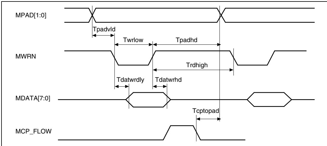
Figure 31.47 MOST Interface Timing (2)
