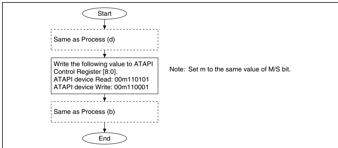
Figure 18.15 Transfer from/to Graphic Memory through Pixel Bus by Polling
