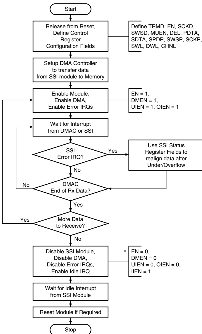
Figure 14.23 Reception using DMA Transfer
