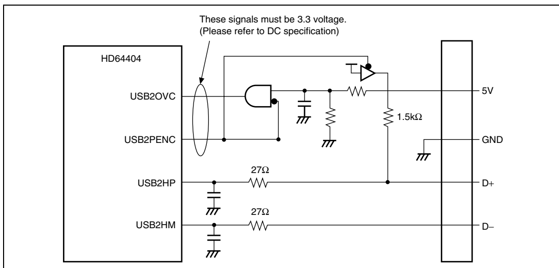
Figure 23.15 Connection Example 1 (When Using USB2PENC)
