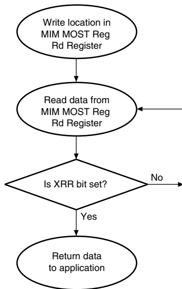
Figure 20.7 Procedure for Reading Transceiver Registers
