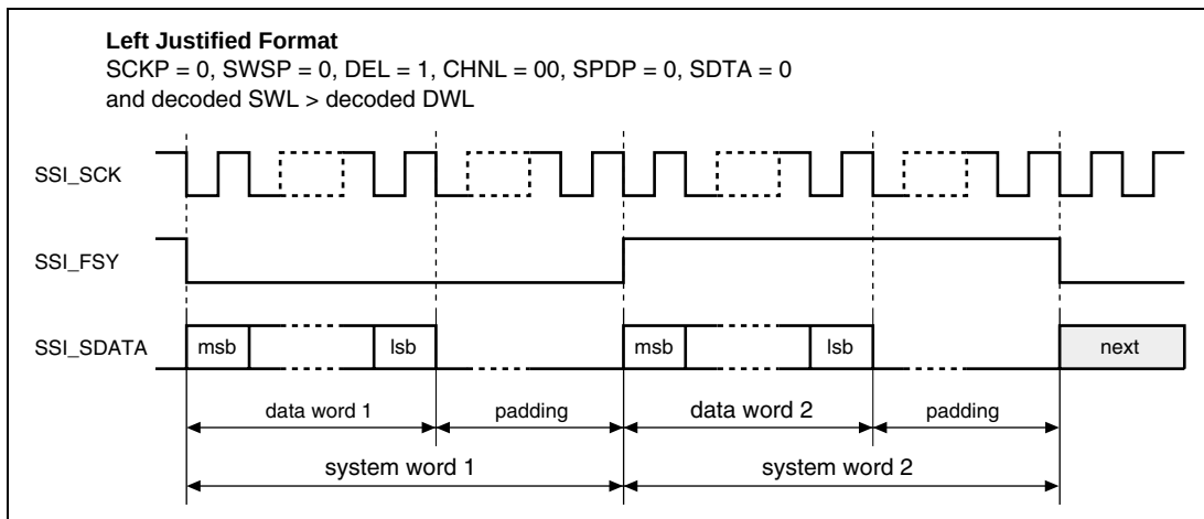
Figure 14.4 Sony Format (Left Justified)
