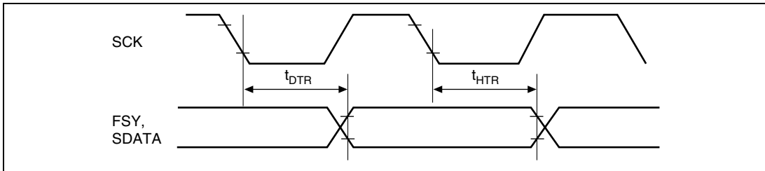
Figure 31.36 Timing for SSI Transmitter (2)
