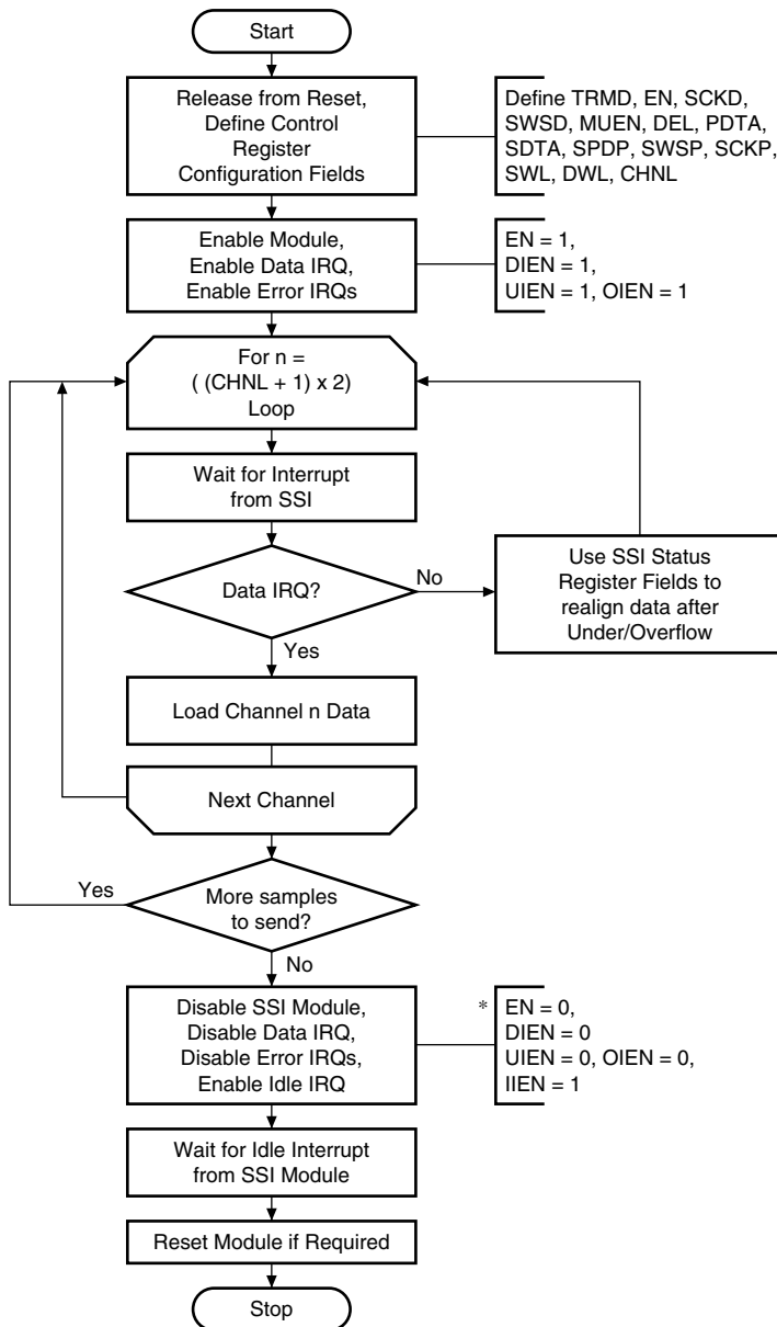
Figure 14.22 Transmission using IRQ Data Flow Control
