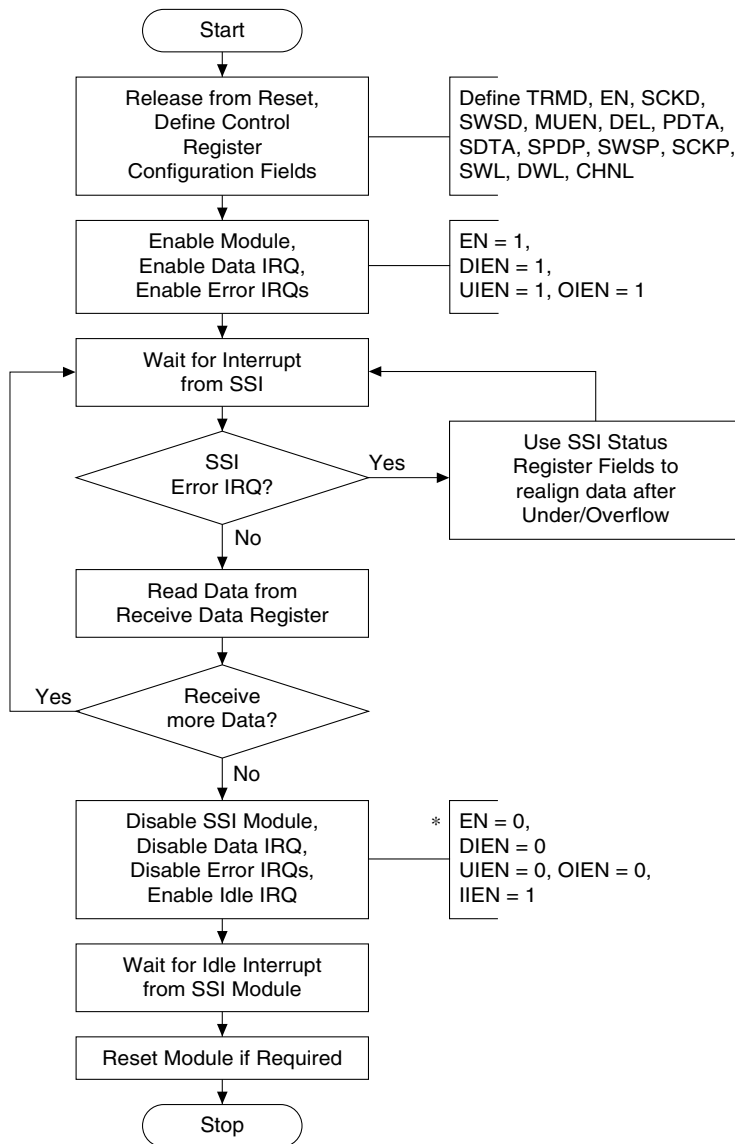
Figure 14.24 Reception using IRQ Flow Control
