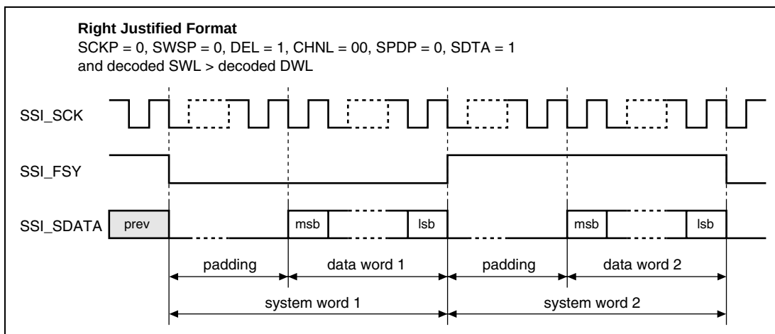
Figure 14.5 Matsushita Format (Right Justified)
