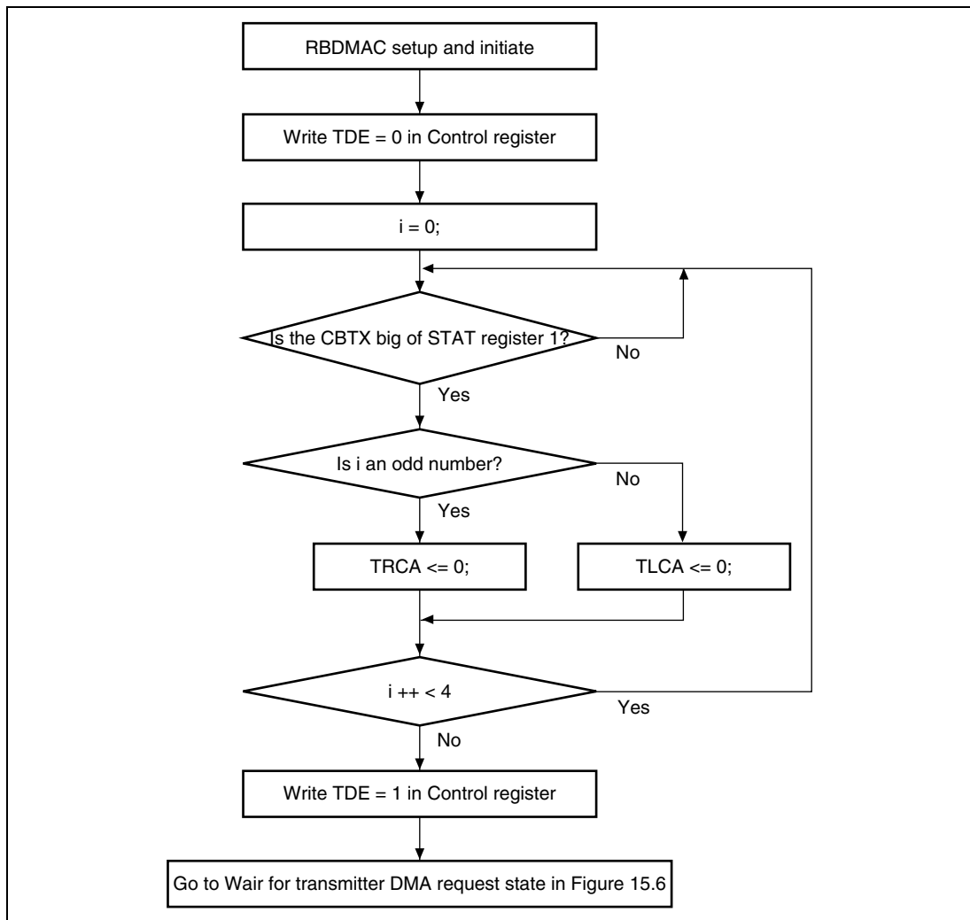
Figure 15.9 Transmitter Data Transfer Flow Diagram – DMA request Driven in case rblck is more than 40MHz
