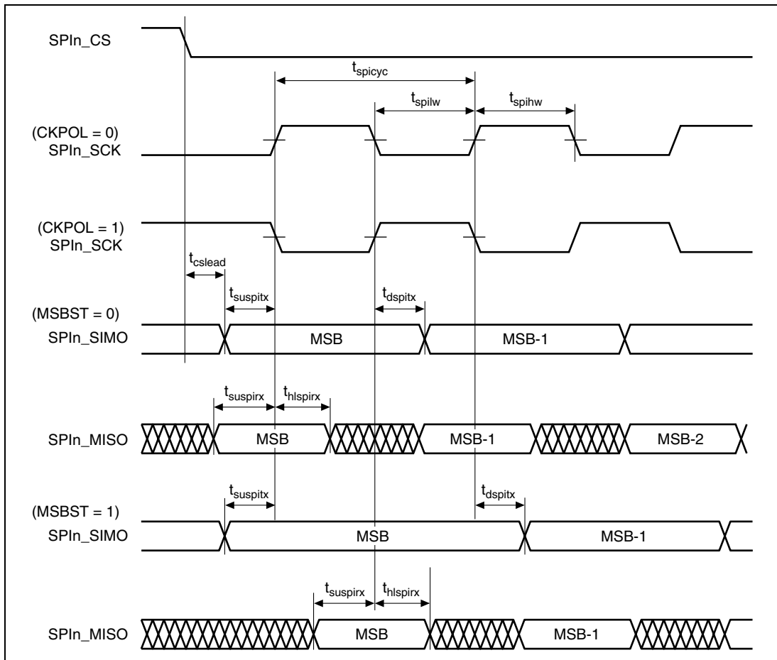
Figure 31.45 SPI Data Output/Input Timing
