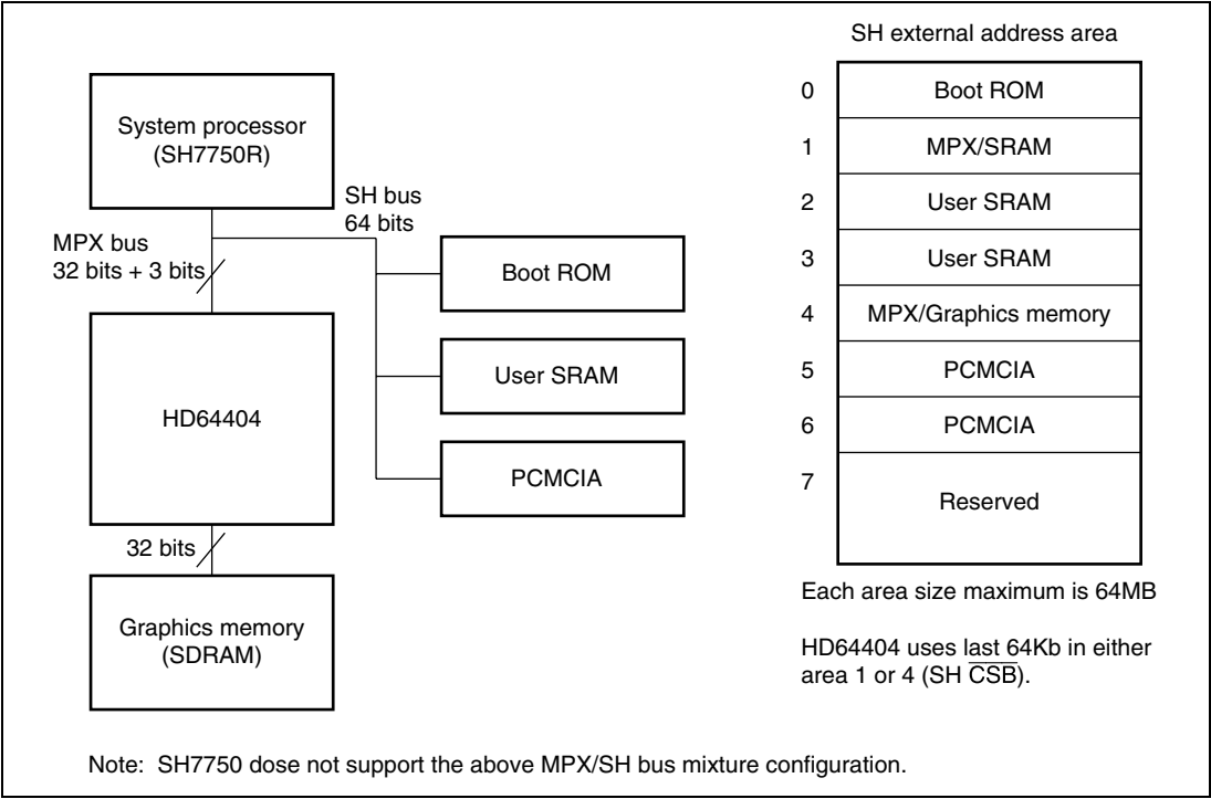
Figure 1.7 MPX System Example 2
