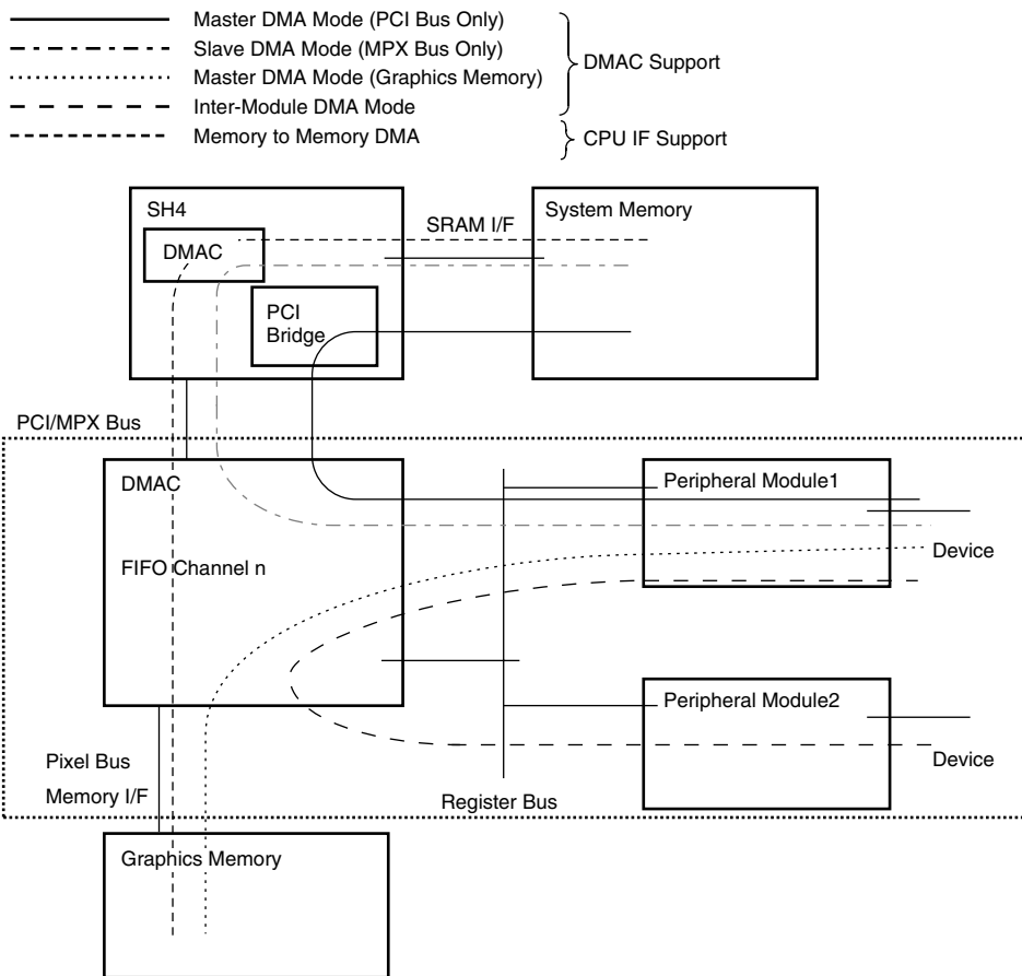
Figure 2.2 HD64404 DMA Data paths
