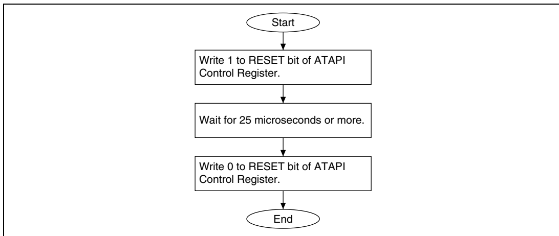
Figure 18.17 Procedure in Hardware Reset for ATAPI Device
