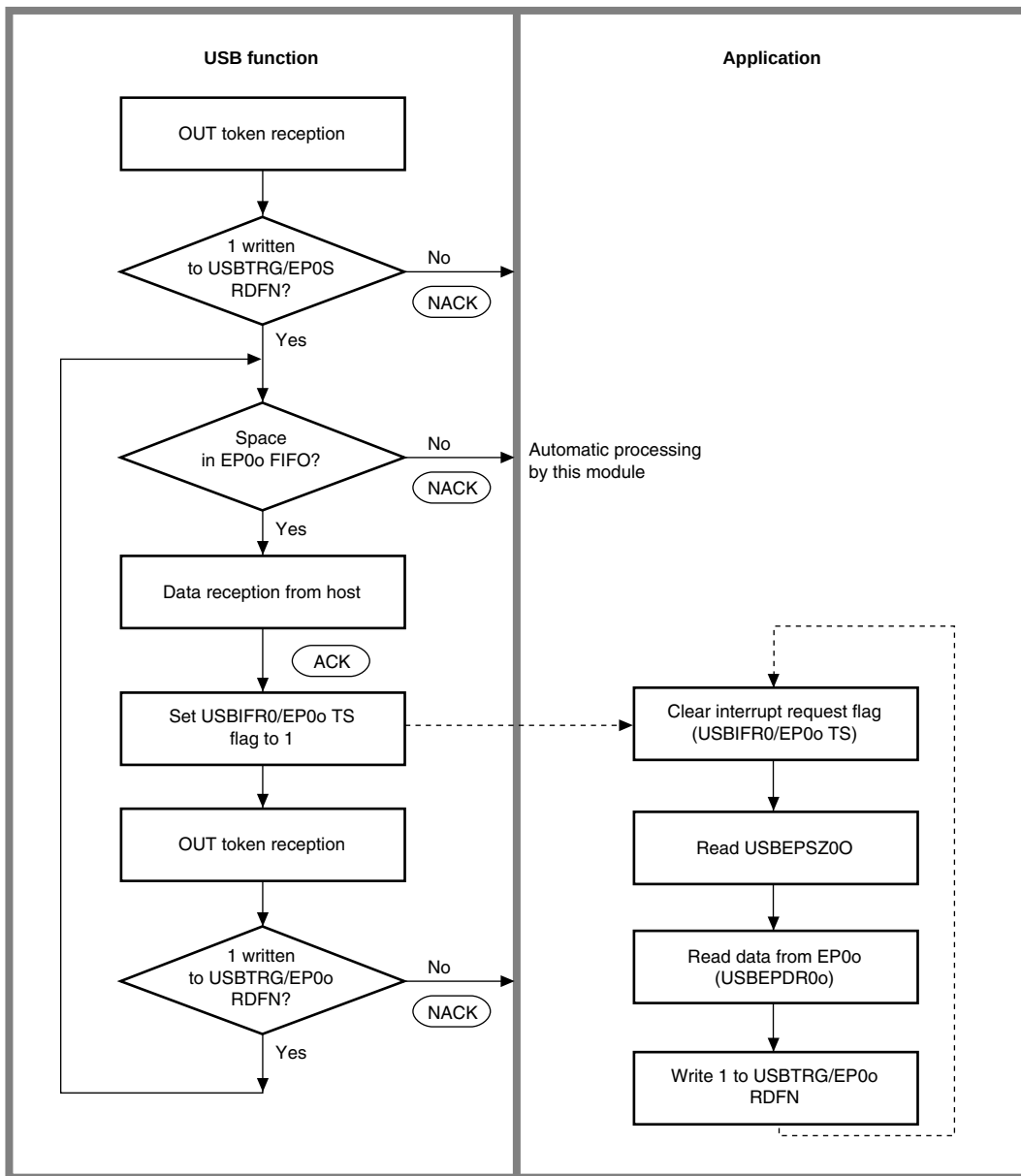
Figure 23.6 Data Stage (Control-Out Transfer Operation)
