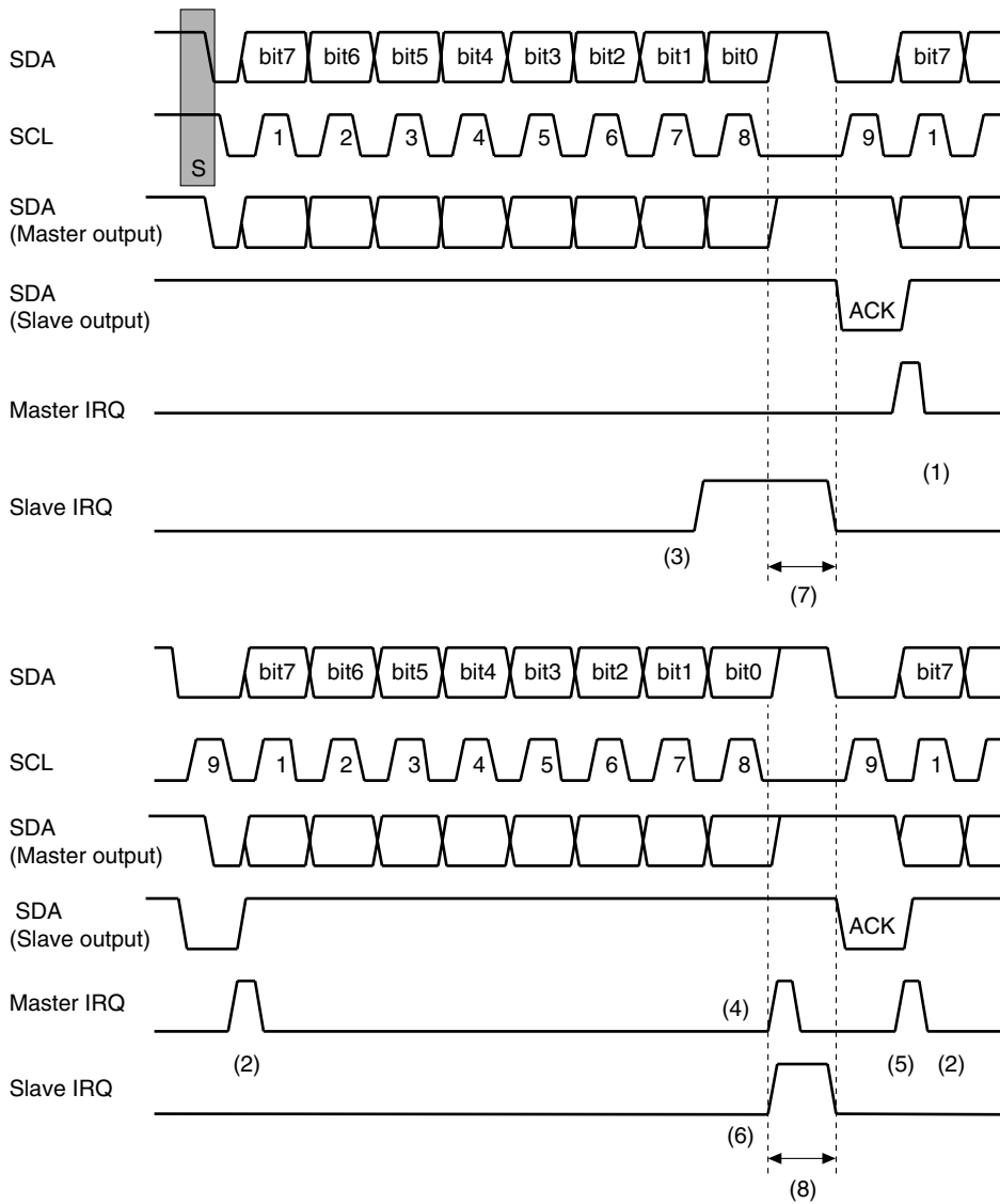
Figure 16.10 Data Transmit Mode Operation Timing
