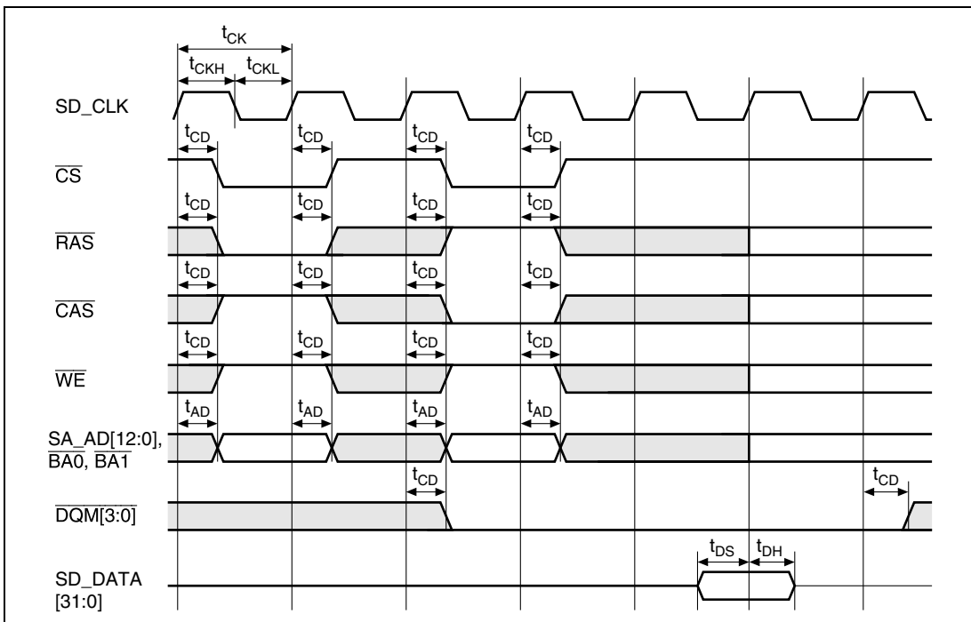
Figure 31.12 SDRAM Read Cycle
