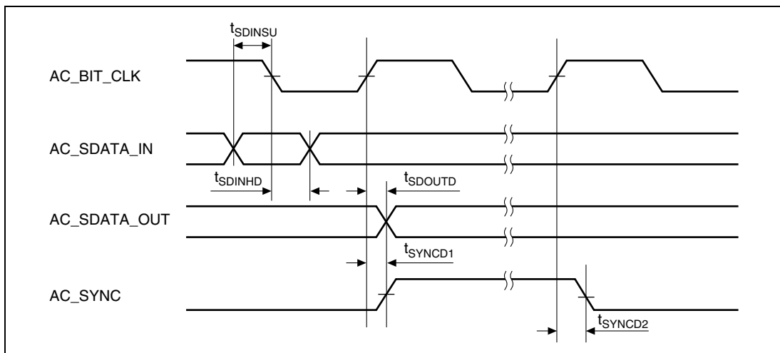
Figure 31.50 Audio Codec Interface Timing
