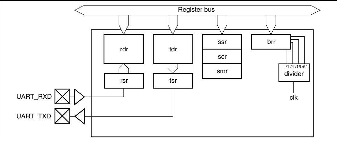
Figure 21.2 Functional Block Diagram
