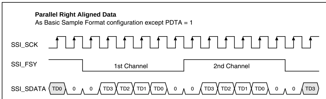
Figure 14.16 Parallel Right Aligned with Delay
