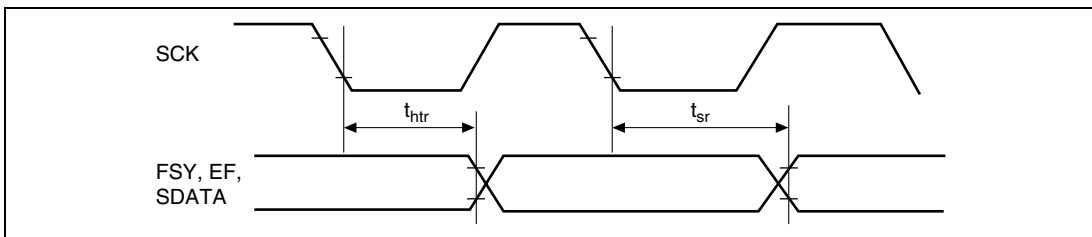
Figure 31.38 Timing for SSI Receiver (2)
