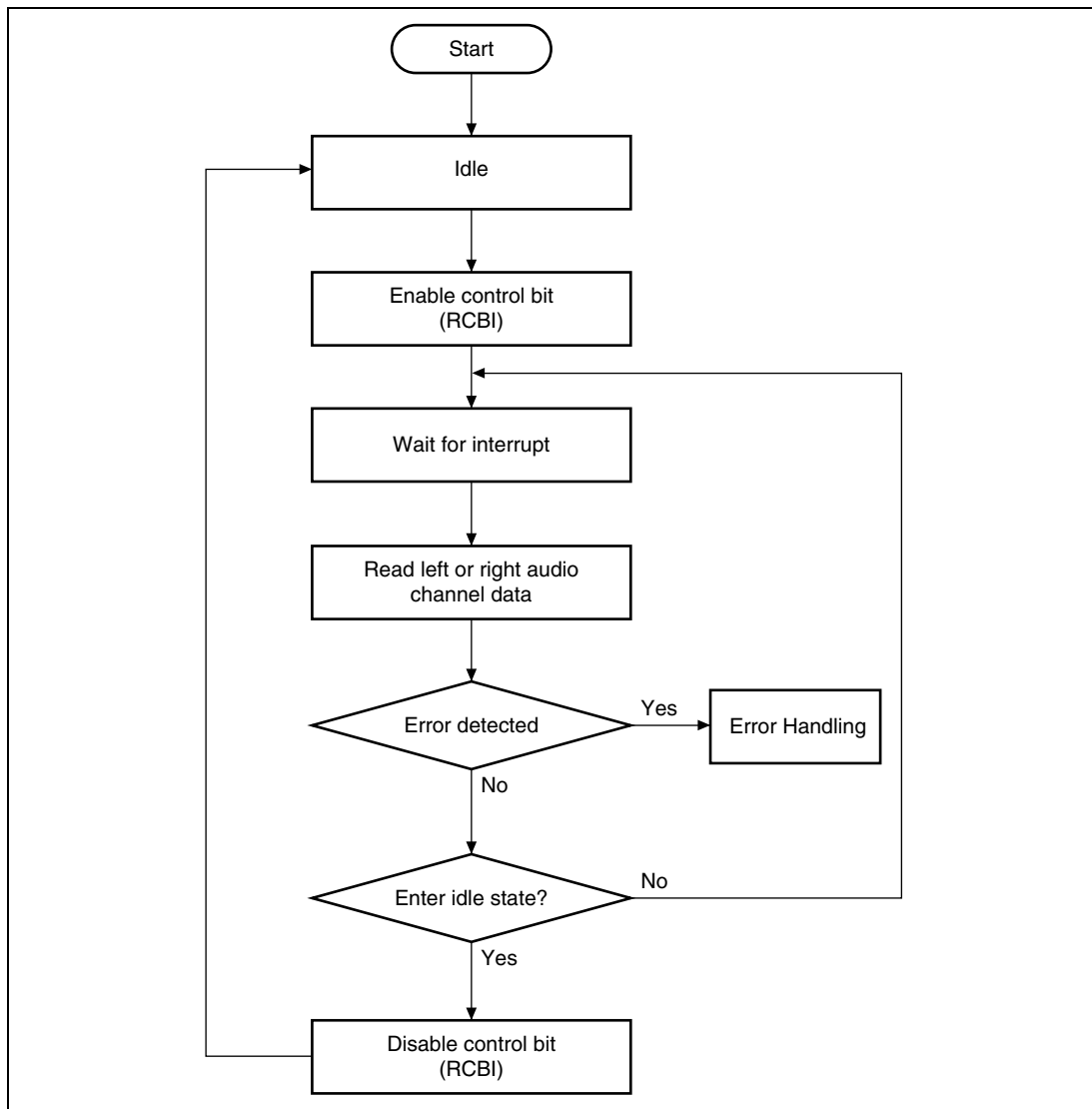
Figure 15.8 Receiver Data transfer Flow Diagram - Interrupt Driven
