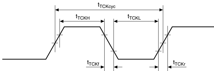
Figure 31.51 TCK Input Timing
