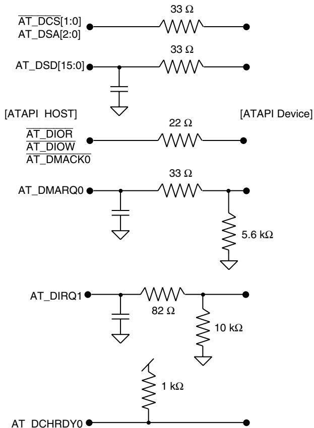
Figure 18.5 Required Termination
