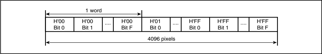
Figure 11.14 Configuration of One Memory Unit (512 Bytes) (1)
