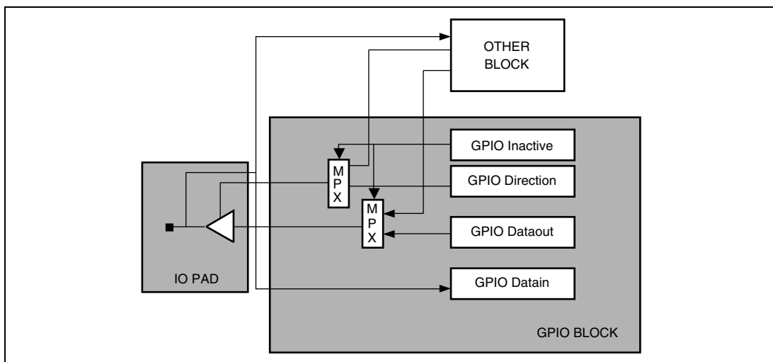
Figure 28.1 GPIO Block Diagram
