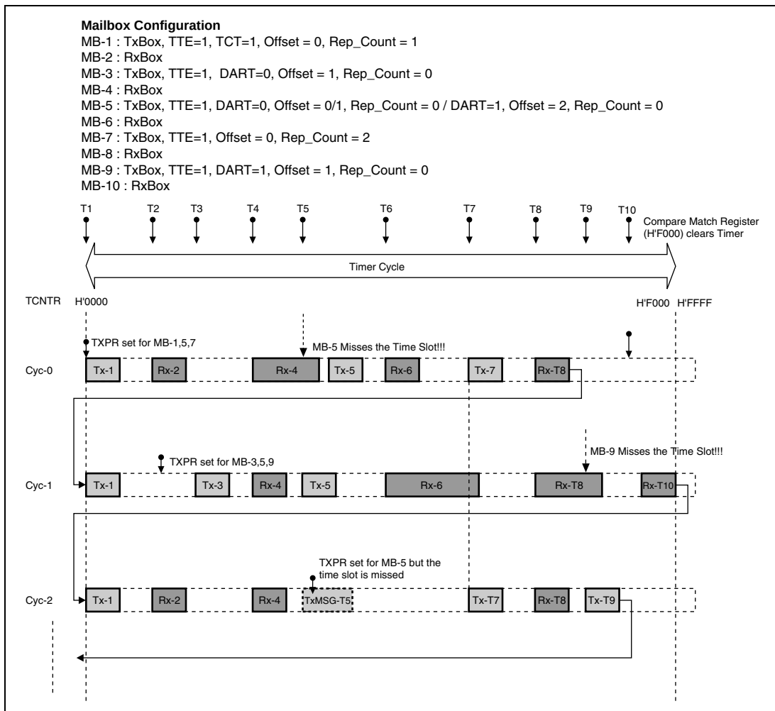
Figure 19.11 Example of Time Triggered System
