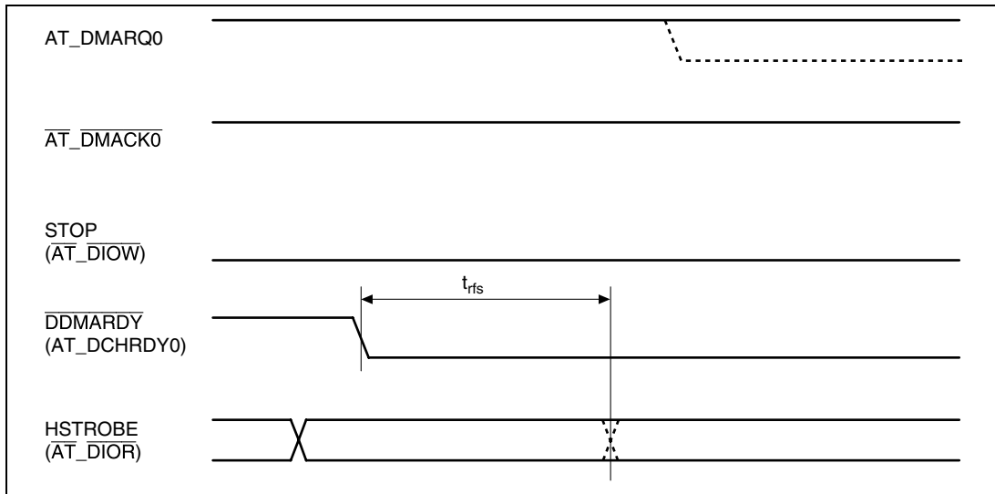
Figure 31.31 Device Pausing an Ultra DMA Data-out Burst
