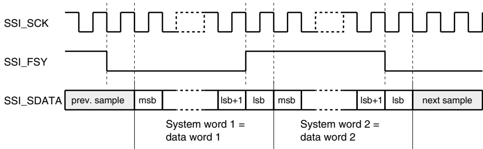
Figure 14.2 Philips Format (with no Padding)
