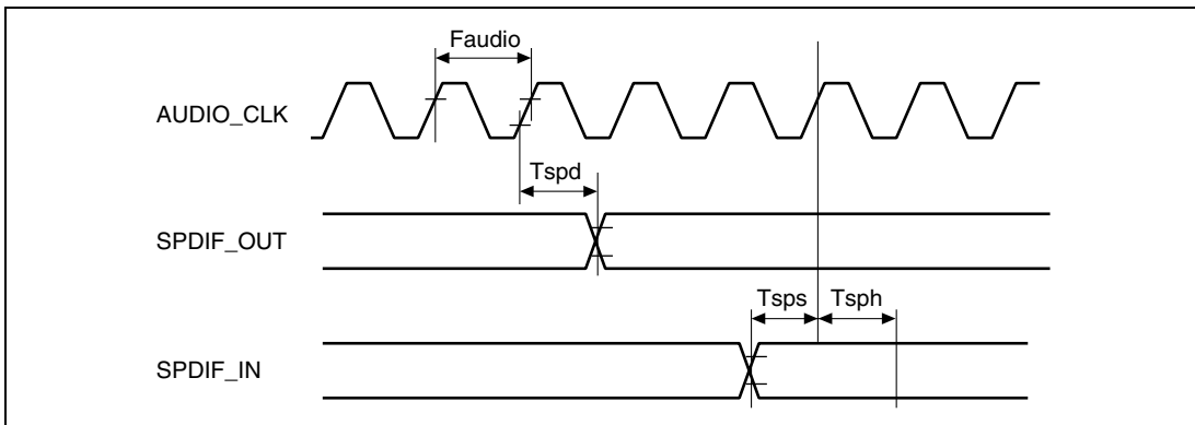
Figure 31.21 SPDIF Timing
