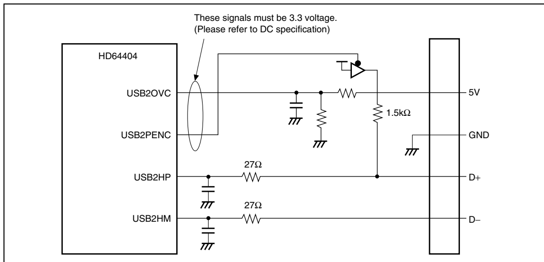
Figure 23.16 Connection Example 2 (When Using USB2PENC)
