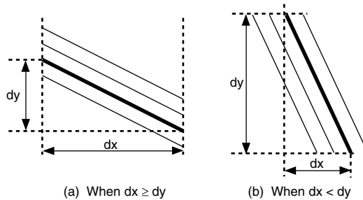
Figure 11.37 Examples of Bold Line Drawing (Line Width 4 Drawing) ( FWUL = 1 , FWDR = 1 )
