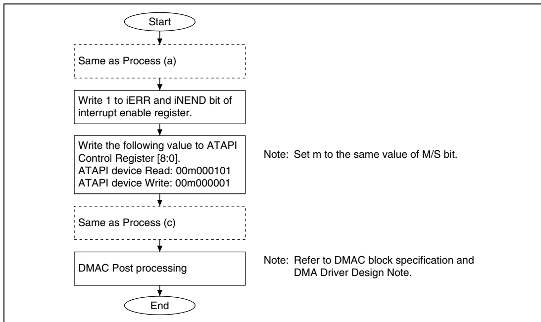
Figure 18.10 Transfer from/to Peripherals on Register Bus by Interrupt
