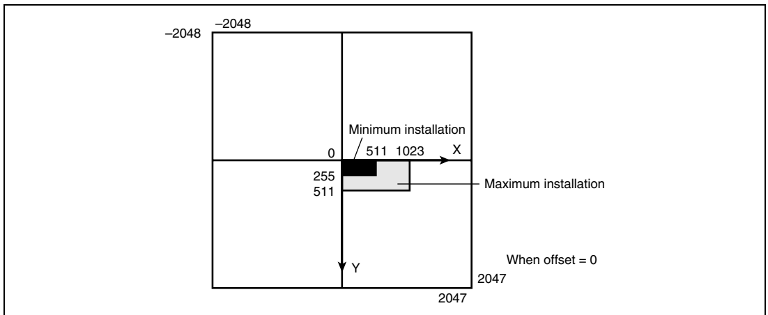
Figure 11.22 Rendering Coordinates
