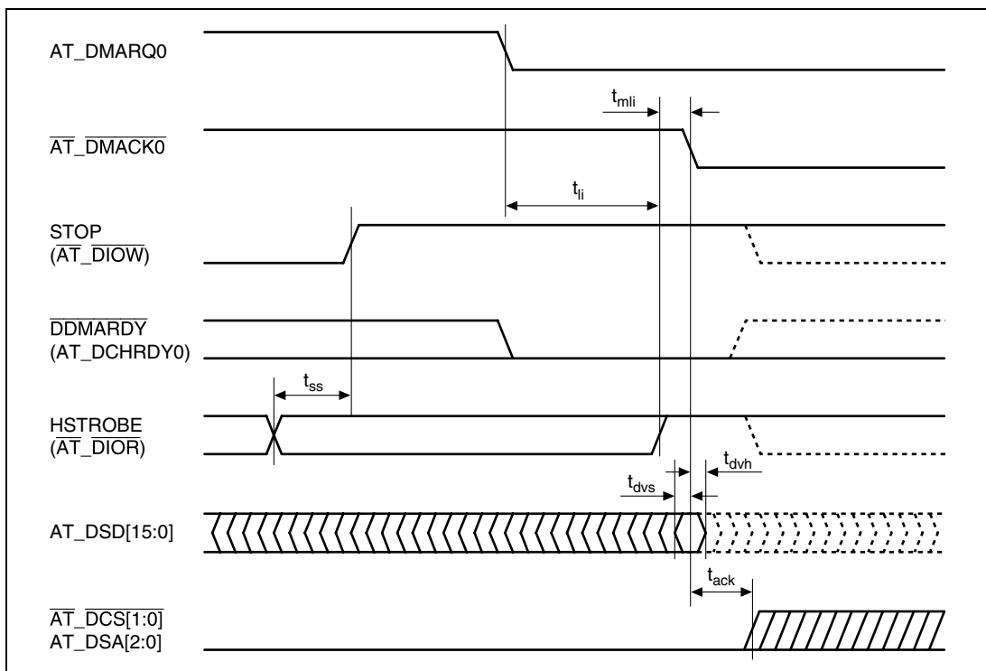
Figure 31.32 Host Terminating an Ultra DMA Data-out Burst
