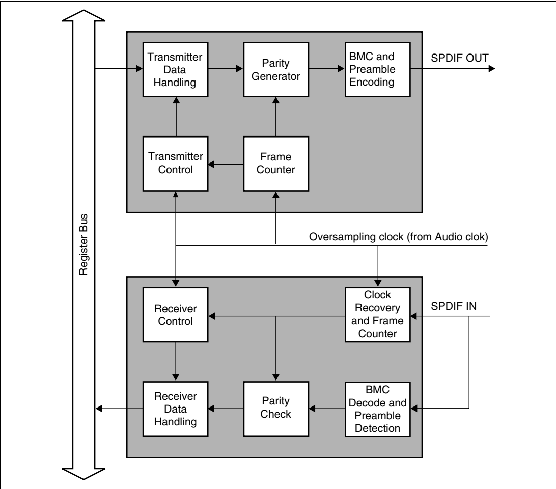
Figure 15.2 Functional Block Diagram
