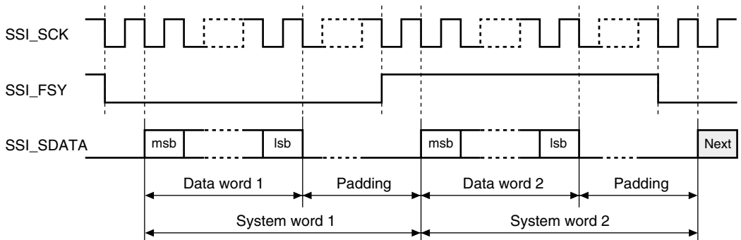
Figure 14.3 Philips Format (with Padding)
