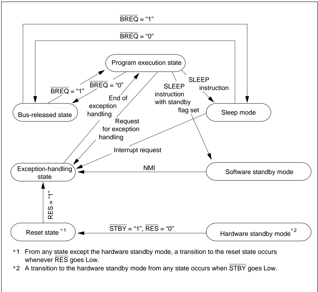
Figure 3-12 State Transitions
