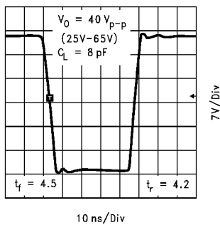
FIGURE 5. Pulse Response
