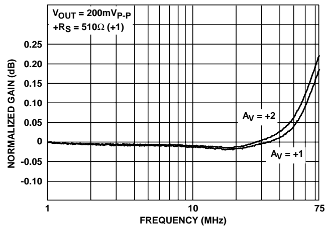
FIGURE 18. GAIN FLATNESS
