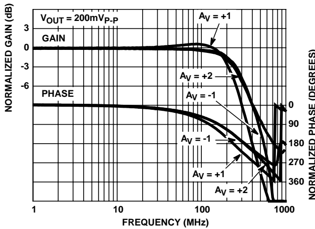
FIGURE 18. FREQUENCY RESPONSE
