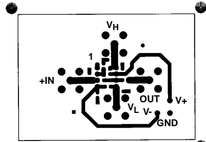
BOTTOM LAYOUT
