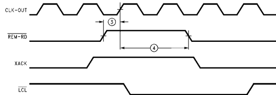
(b) REM-RD Rest Time (Latched Read Mode)
