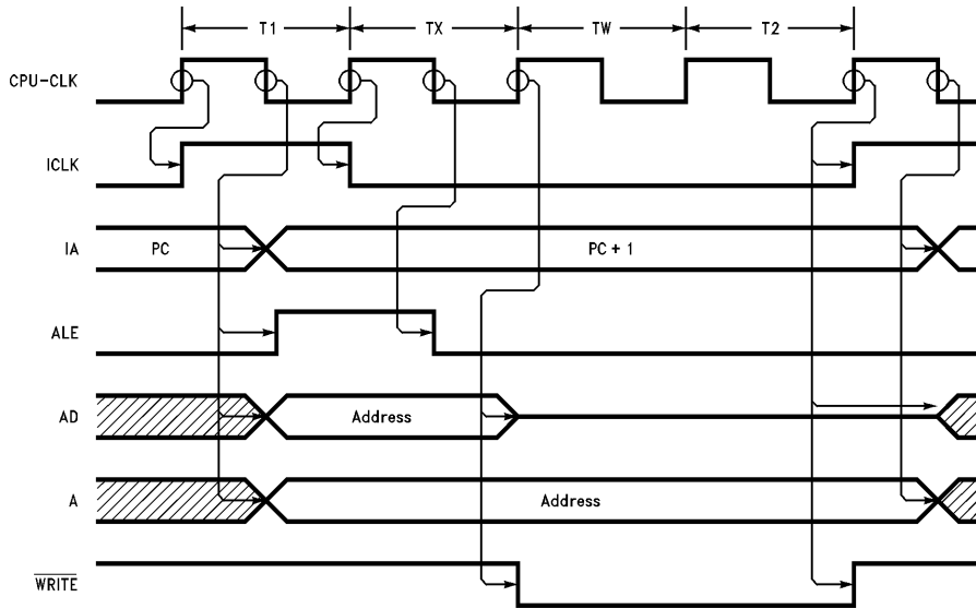
FIGURE 2-22. Data Memory Read with One Wait State and [4TR] = 0
