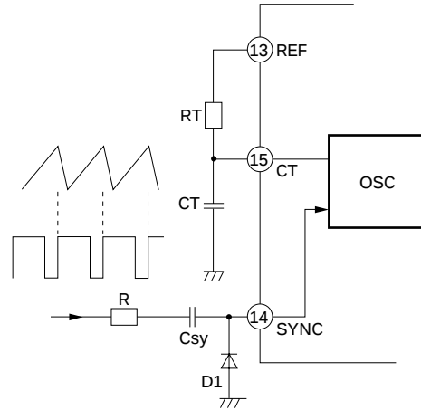
Fig. 1 Oscillator
