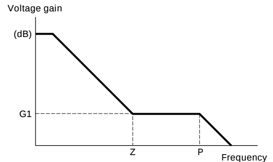
Fig. 4 Voltage gain-frequency
