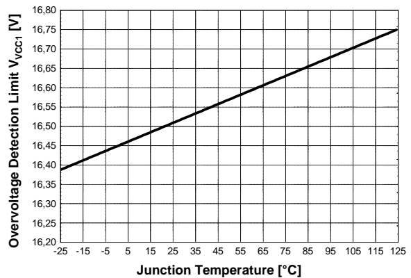
Figure 40 Overvoltage Detection Limit V_{VCC1} vs. T_j
