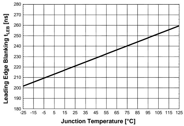
Figure 42 Leading Edge Blanking V_{VCC1} vs. T_j
