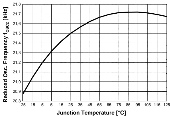
Figure 31 Reduced Osc. Frequency f_{OSC2} vs. T_j
