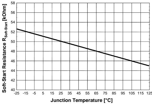
Figure 36 Soft-Start Resistance R_{Soft-Start} vs. T_j
