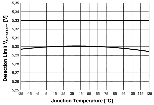
Figure 38 Detection Limit V_{Soft-Start1} vs. T_j
