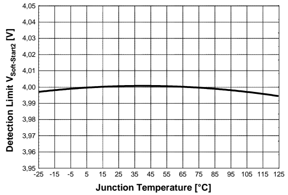
Figure 39 Detection Limit V_{Soft-Start2} vs. T_j
