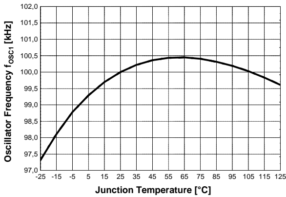
Figure 30 Oscillator Frequency f_{OSC1} vs. T_j
