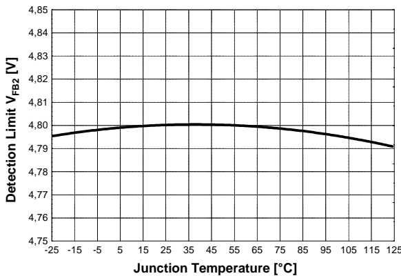
Figure 37 Detection Limit V_{FB2} vs. T_j
