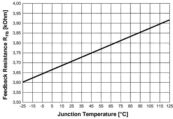
Figure 35 Feedback Resistance R_{FB} vs. T_j
