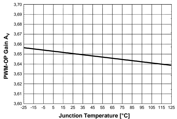
Figure 34 PWM-OP Gain A_V vs. T_j
