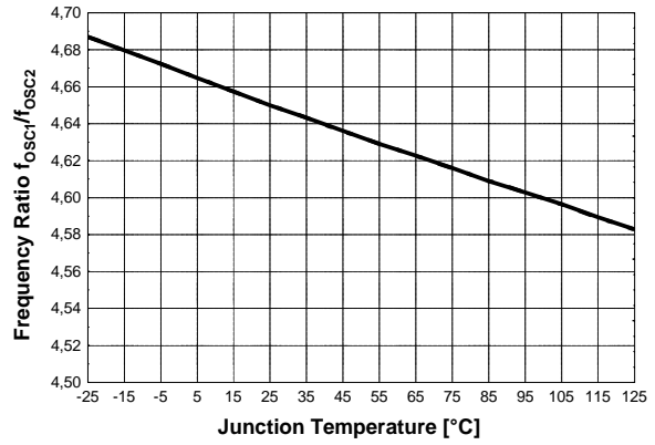
Figure 32 Frequency Ratio f_{OSC1}/f_{OSC2} vs. T_j
