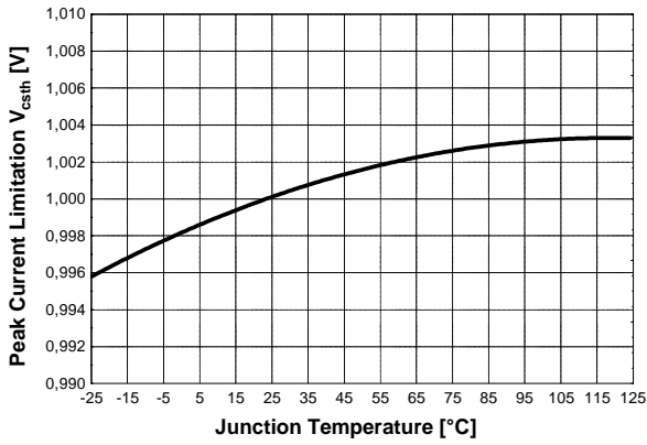
Figure 41 Peak Current Limitation V_{csth} vs. T_j
