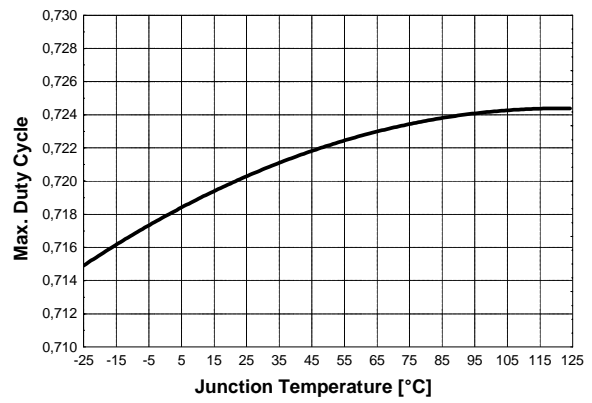
Figure 33 Max. Duty Cycle vs. T_j
