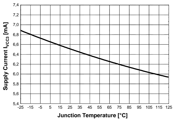
Figure 25 Supply Current I_{VCC3} vs. T_j
