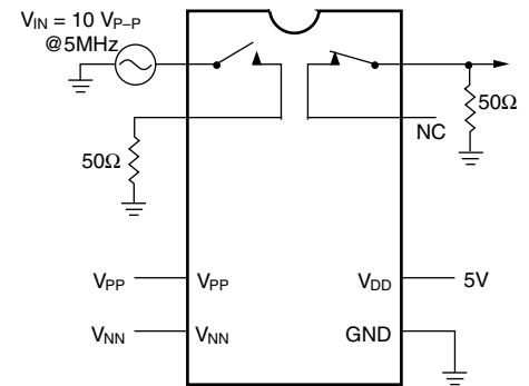
Crosstalk
