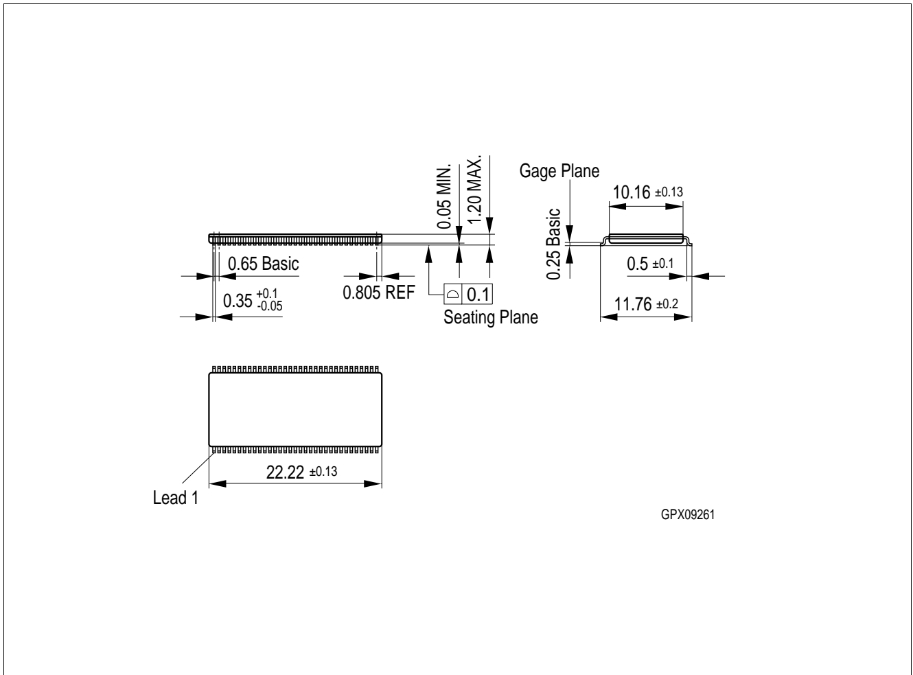
Figure 52 P-TSOPII-66-1 (Plastic Thin Small Outline Package Type II)
