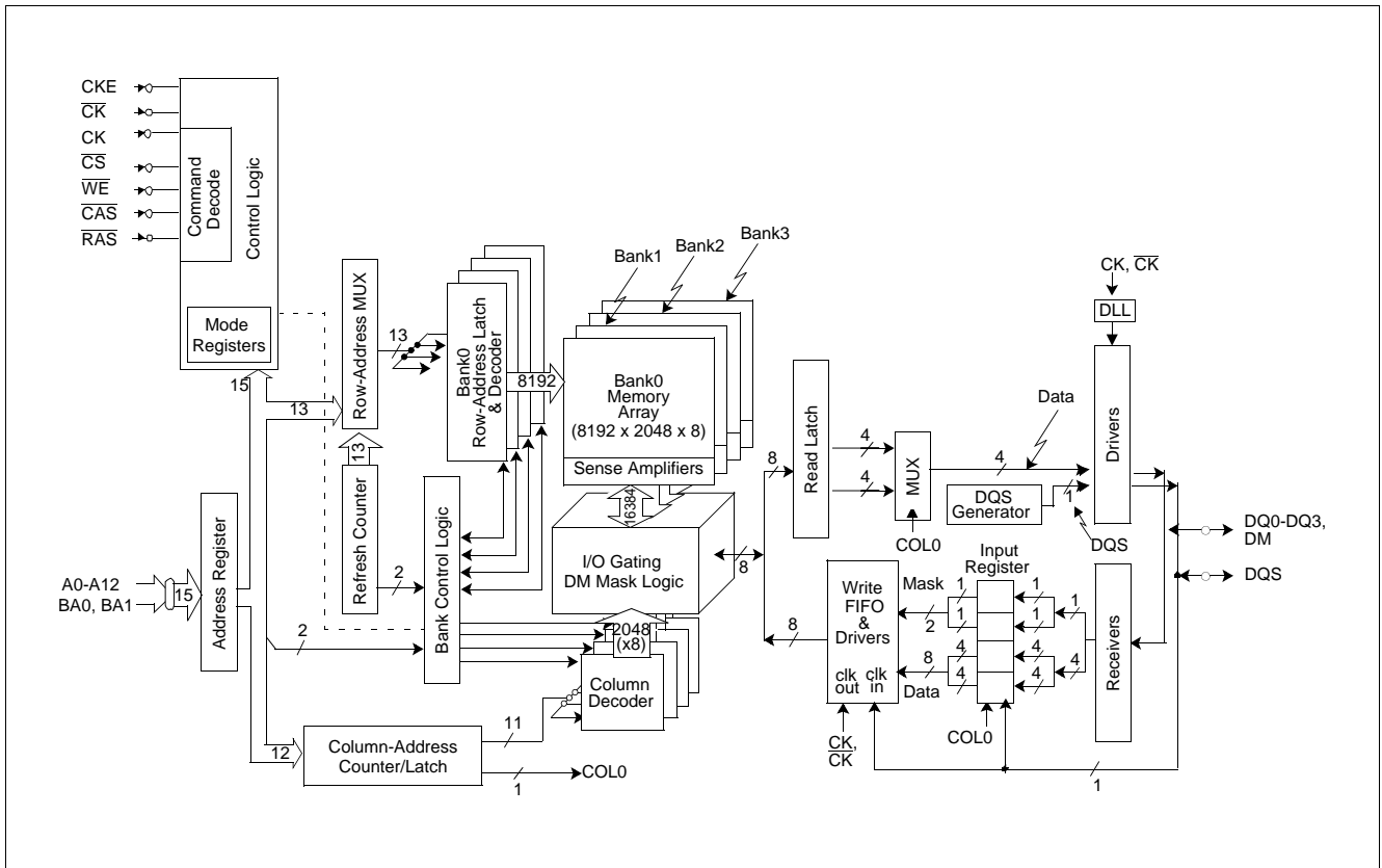
Figure 3 Block Diagram (128 Mbit × 4)
