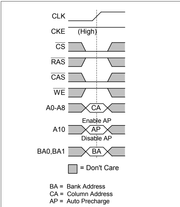
Figure 14 READ Command
