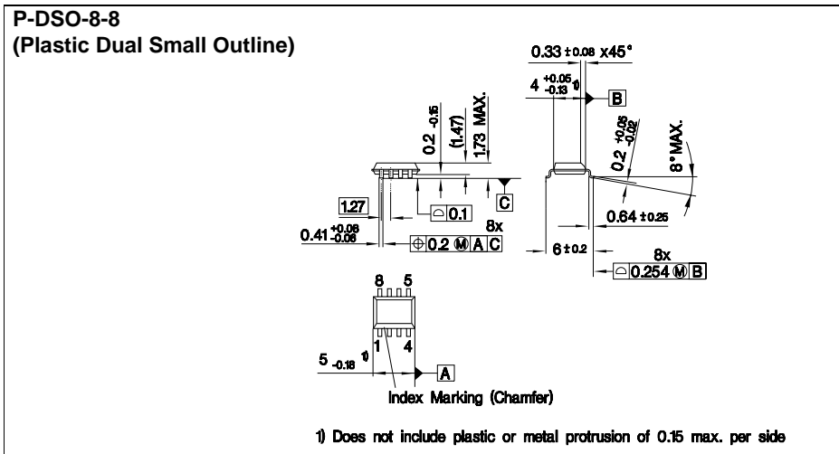
Figure 22 P-DSO-8-8 (Plastic Dual Small Outline)
