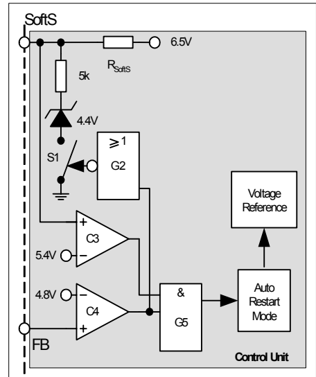
Figure 20 Auto Restart Mode
