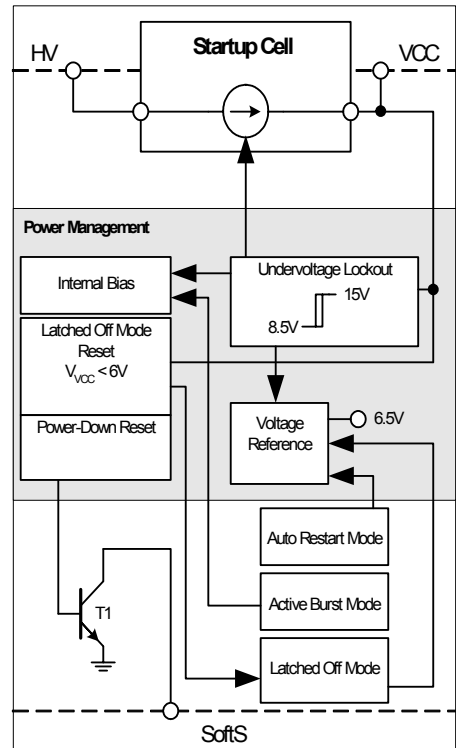
Figure 4 Power Management
