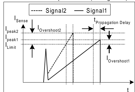
Figure 12 Current Limiting
