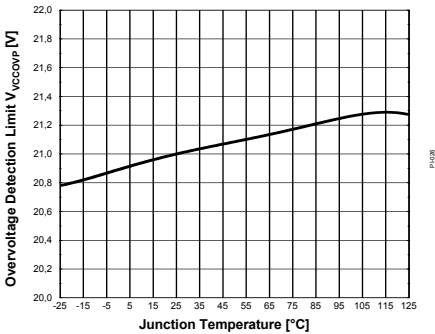
Figure 46 Overvoltage Detection Limit V_{VCCOV}
