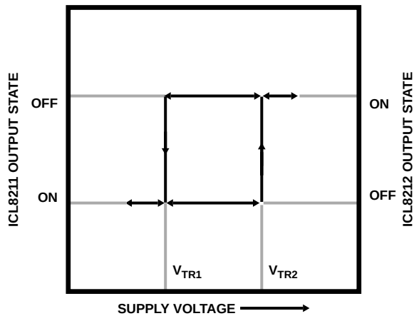
FIGURE 27. TWO ALTERNATIVE VOLTAGE DETECTION CIRCUITS EMPLOYING HYSTERESIS TO PROVIDE PAIRS OF WELL DEFINED TRIP VOLTAGES
