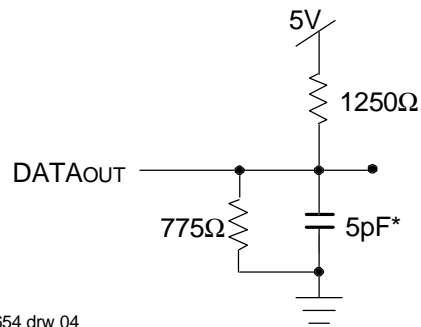
Figure 2. Output Test Load (For t LZ , t RZ , t WZ , t OW ) *Including scope and jig.
