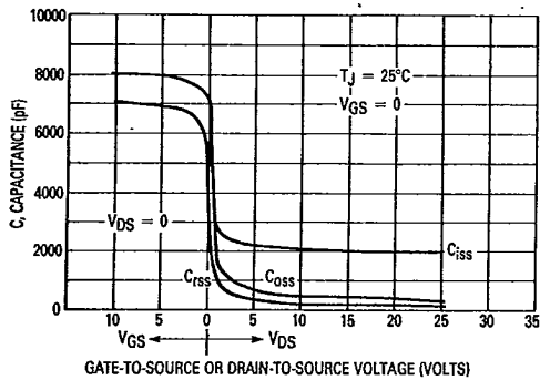
Figure 11. Capacitance Variation
