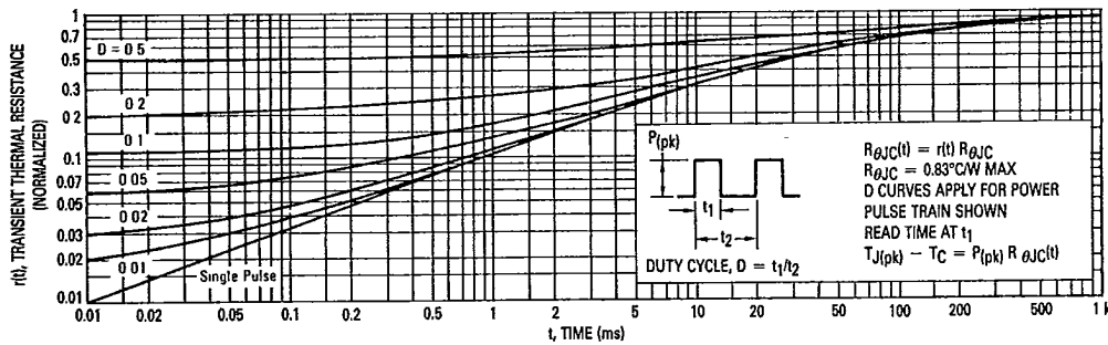
Figure 10. Thermal Response
