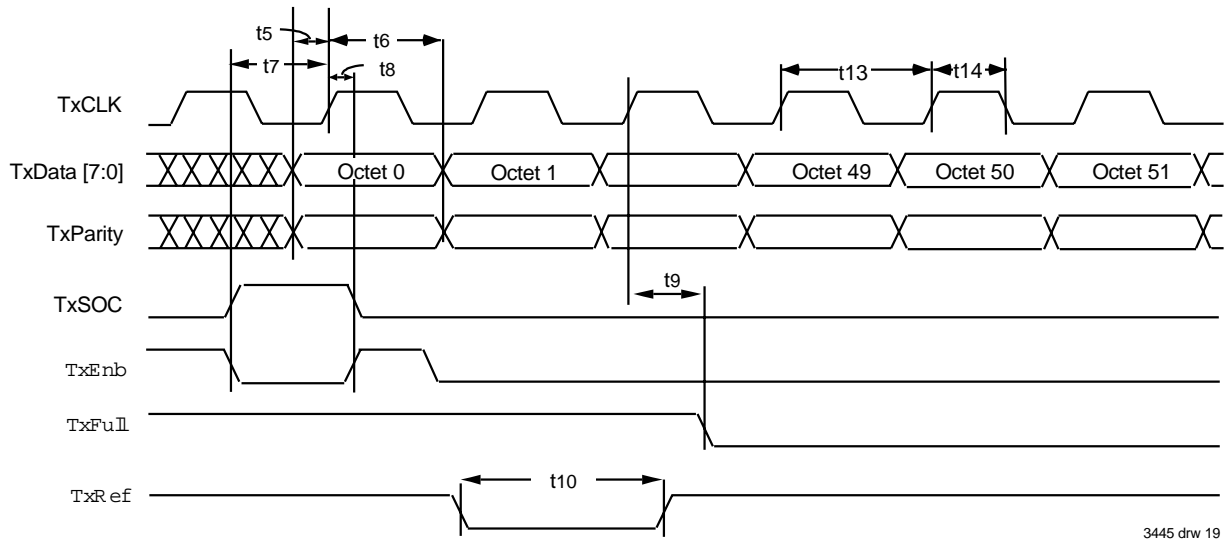
Figure 16 UTOPIA Transmit
