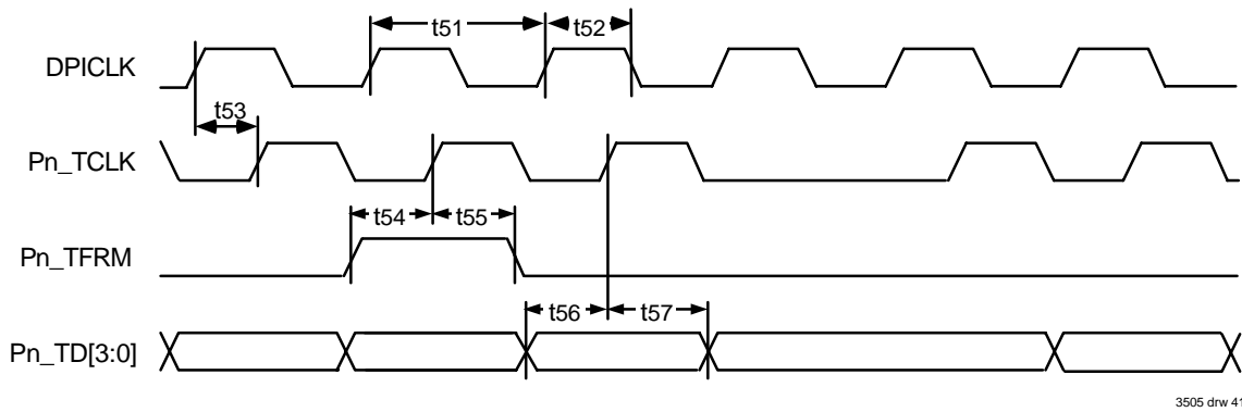
Figure 41 DPI Transmit
