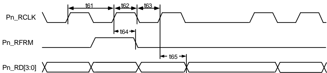
Figure 42 DPI Receive
