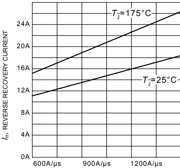
di_F/dt , DIODE CURRENT SLOPE Figure 25. Typical reverse recovery current as a function of diode current slope ( V_R = 400\text{V} , I_F = 20\text{A} , Dynamic test circuit in Figure E)
