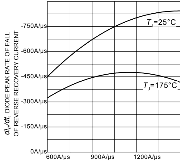
di_F/dt , DIODE CURRENT SLOPE Figure 26. Typical diode peak rate of fall of reverse recovery current as a function of diode current slope ( V_R = 400\text{V} , I_F = 20\text{A} , Dynamic test circuit in Figure E)
