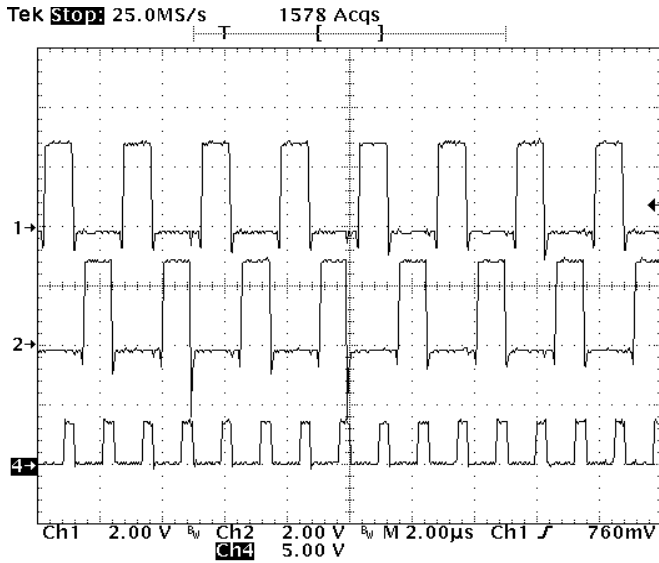
Ch1: Output 1 switching node, 400kHz Ch2: Output 2 switching node, 400kHz Ch3: 800kHz external synchronization Ch4: 800kHz external synchronization
