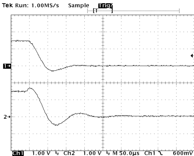
Fig. 25: iP1202 latched overcurrent response (output1 shutdowns due to overload, whereas output2 continues uninterrupted)
