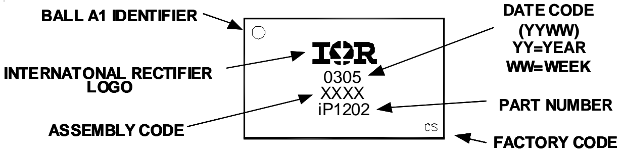
Part Marking
