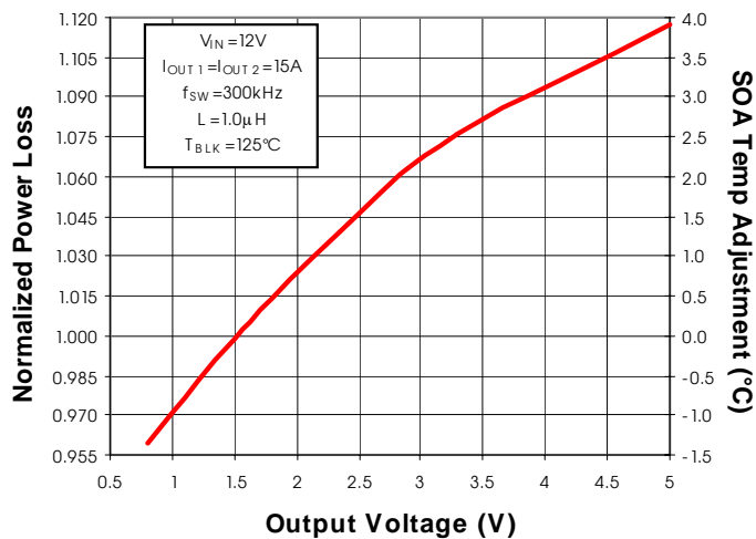
Fig. 5: Normalized Power Loss vs. V_{OUT}
