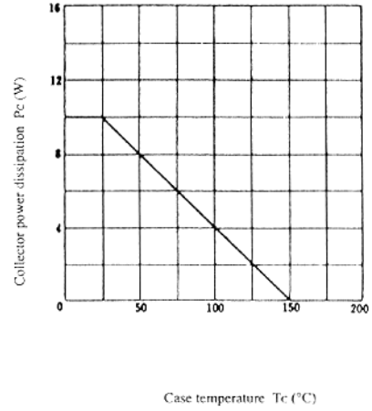
MAXIMUM COLLECTOR DISSIPATION CURVE
